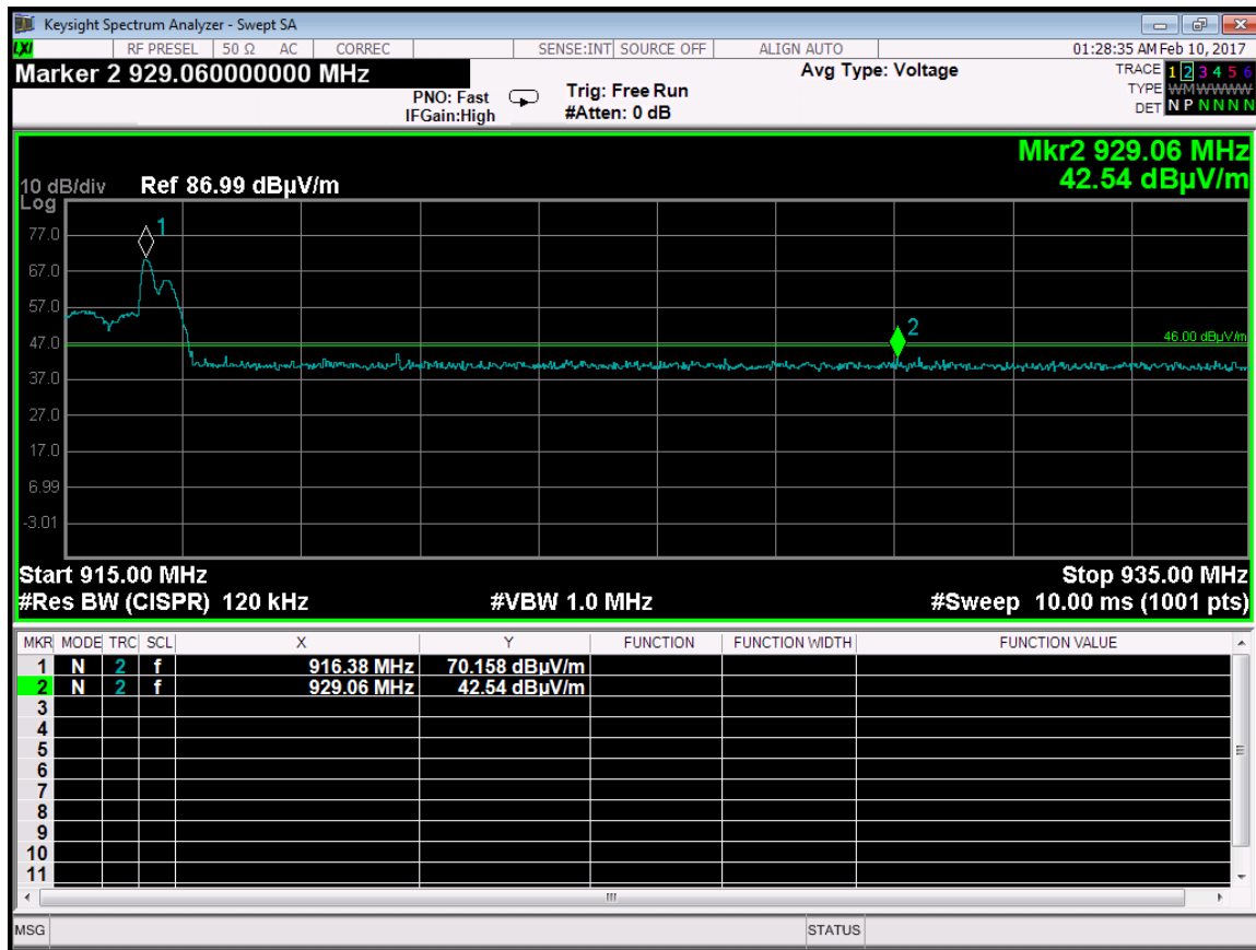
Band Edge – Vertical Polarization-X-Axis Worst Case
