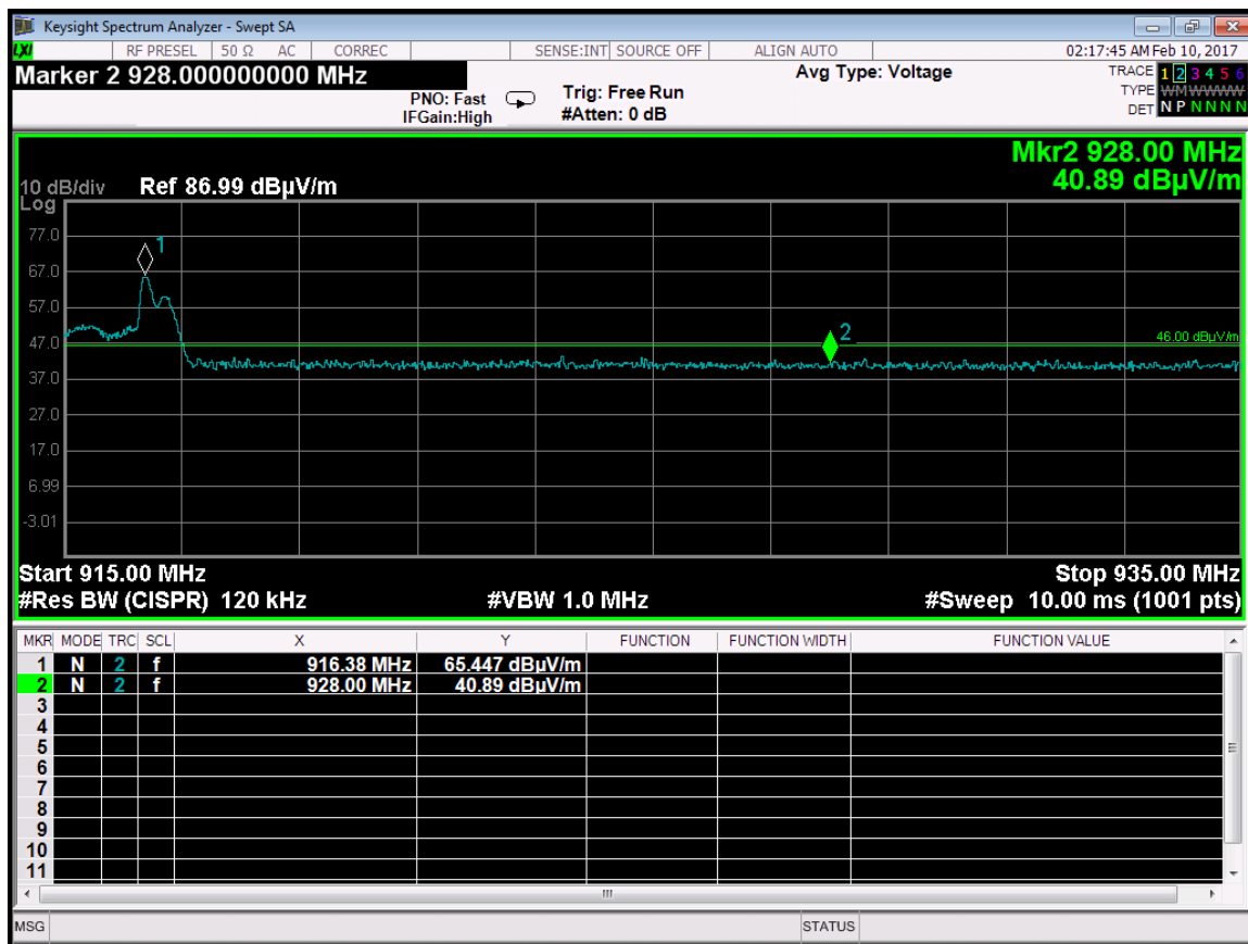
Band Edge – Horizontal Polarization-Z-Axis Worst Case
