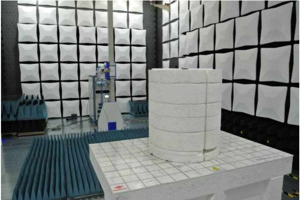
Figure 6: Test Setup for 18 GHz to 26GHz (View 2)
