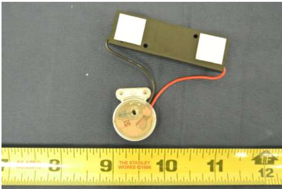
Figure 2: EUT – Bottom View
