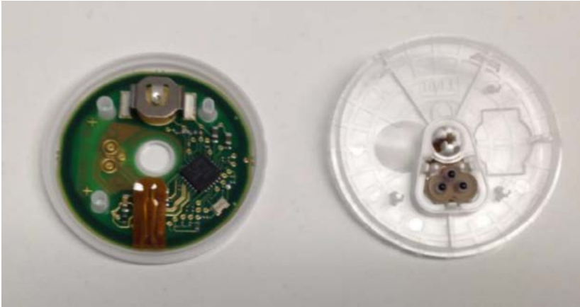
Photo 1- Internal View of the Sensor Top
