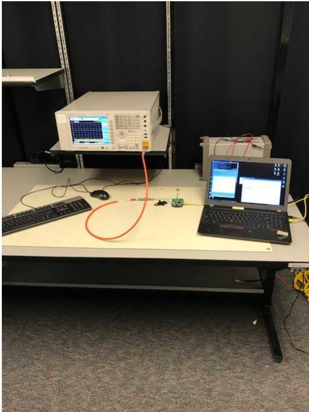
Conducted measurements setup
