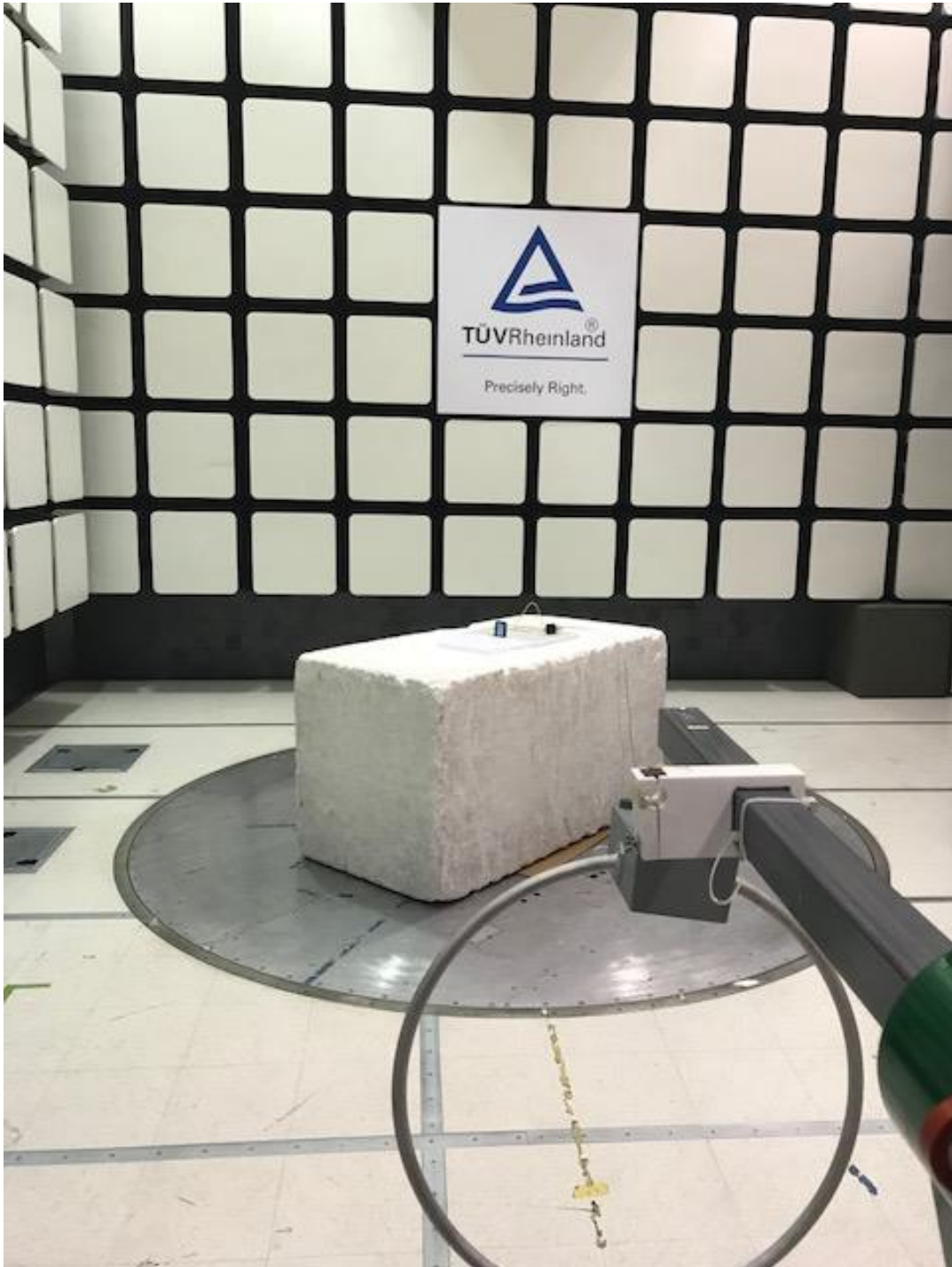
Radiated Emissions 9k-30 MHz front
