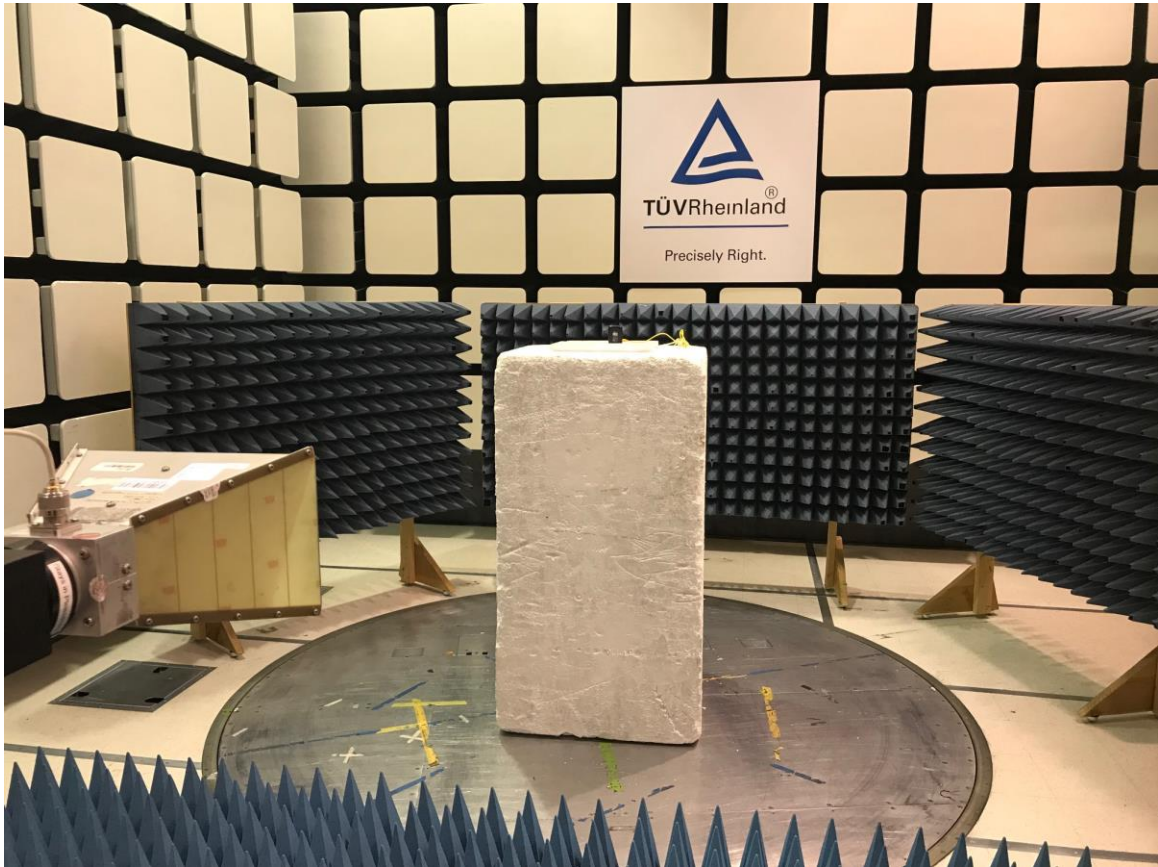
Radiated Emissions 1-18 GHz front
