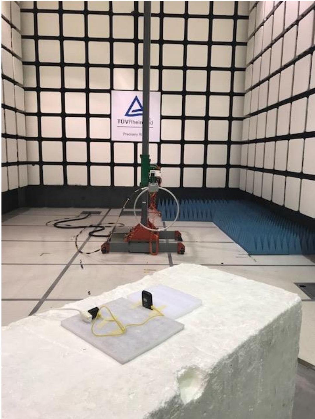
Radiated Emissions 9k-30 MHz rear
