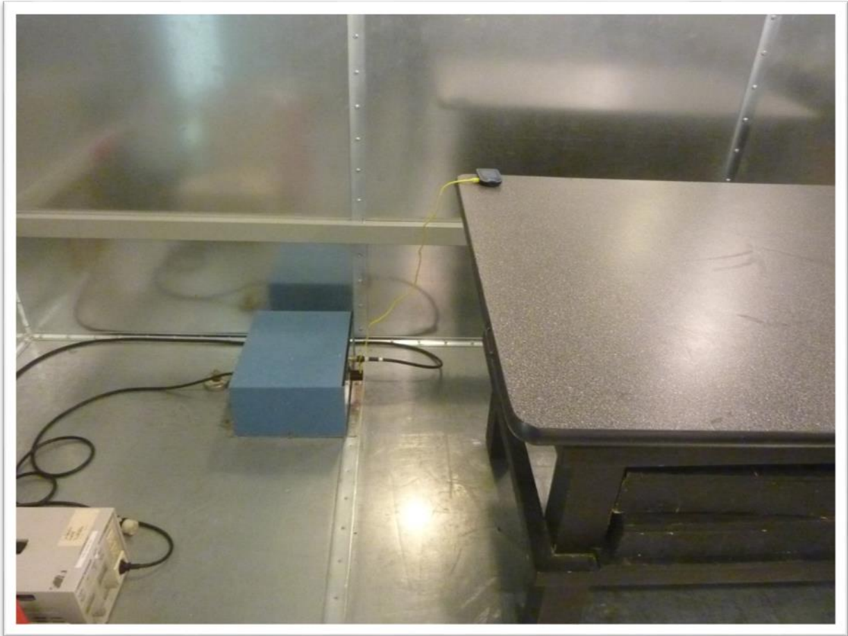
Power line conducted emissions setup
