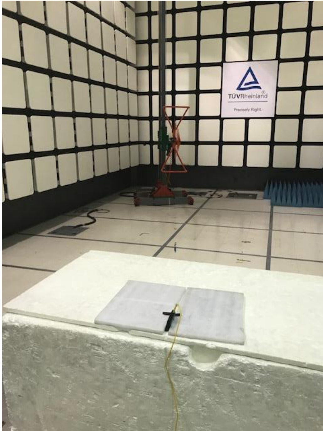
Radiated Emissions 30 to 1GHz rear
