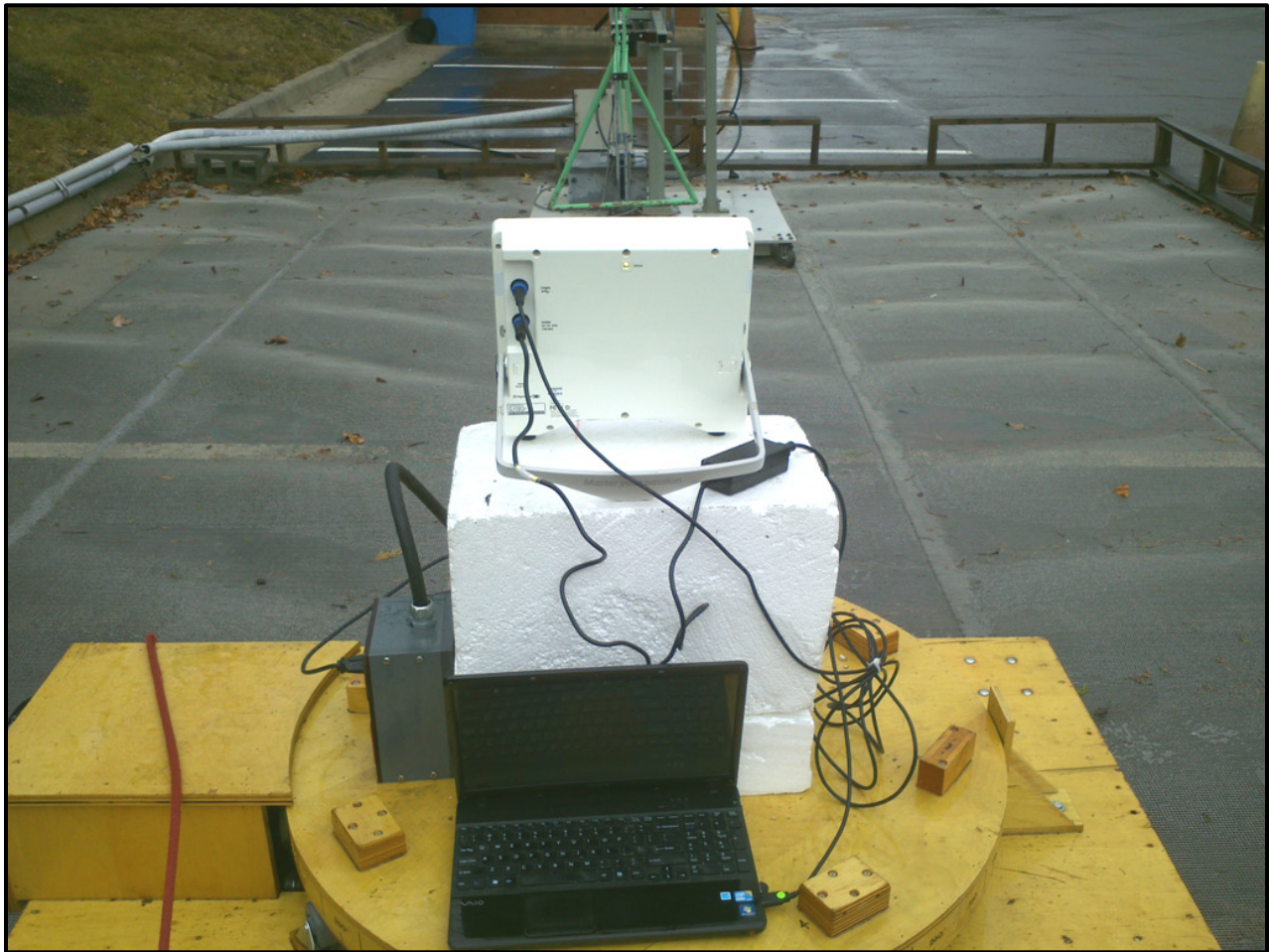
Photograph 2: Radiated Emissions - Rear View
