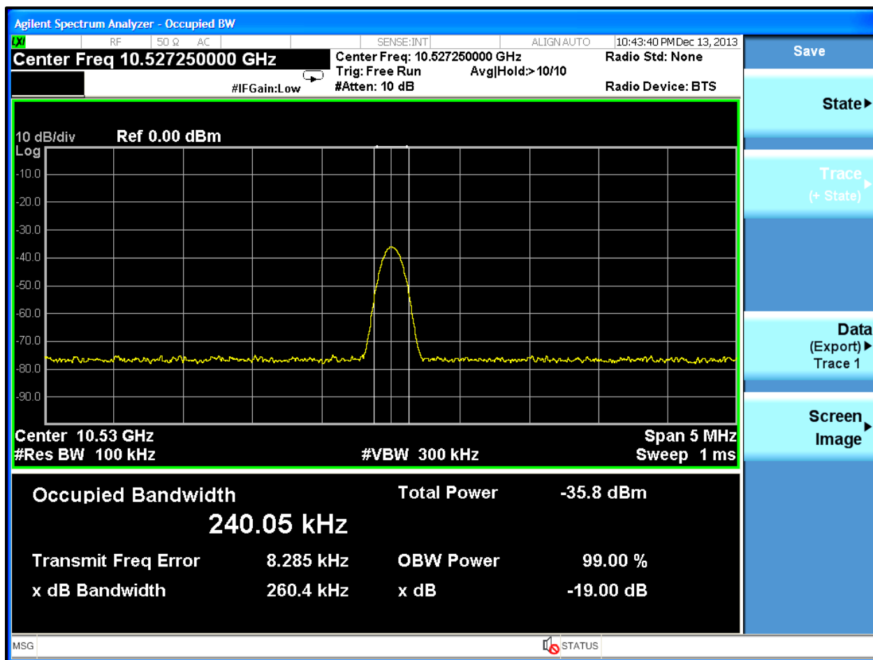
Plot 5-1: 99% Bandwidth
