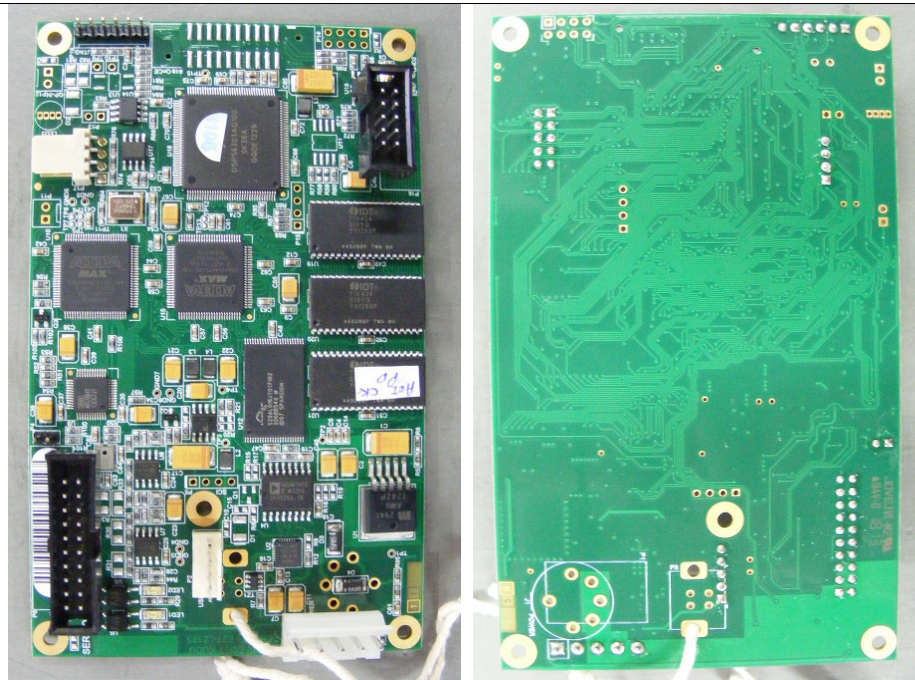
DSP (Digital Signal Processor) PCB – Top and Bottom Views
