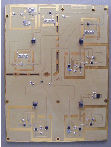
Microwave PBC with integral Tx and Rx antennas – Rear View, without and with screening cans
