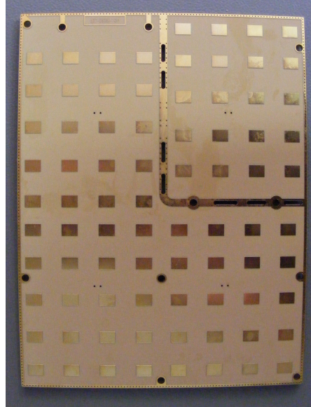
Microwave PBC with integral Tx and Rx antennas – Front View (Antennas)
