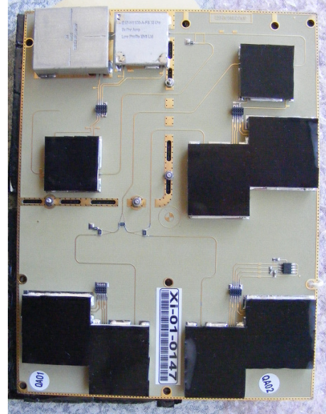
Microwave PBC with integral Tx and Rx antennas – Rear View, without and with screening cans
