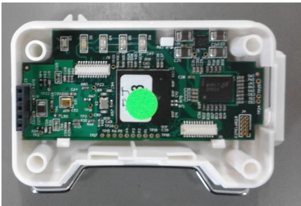
PCB "A" Inserted
