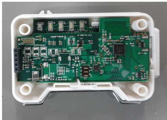
PCB "B" Inserted
