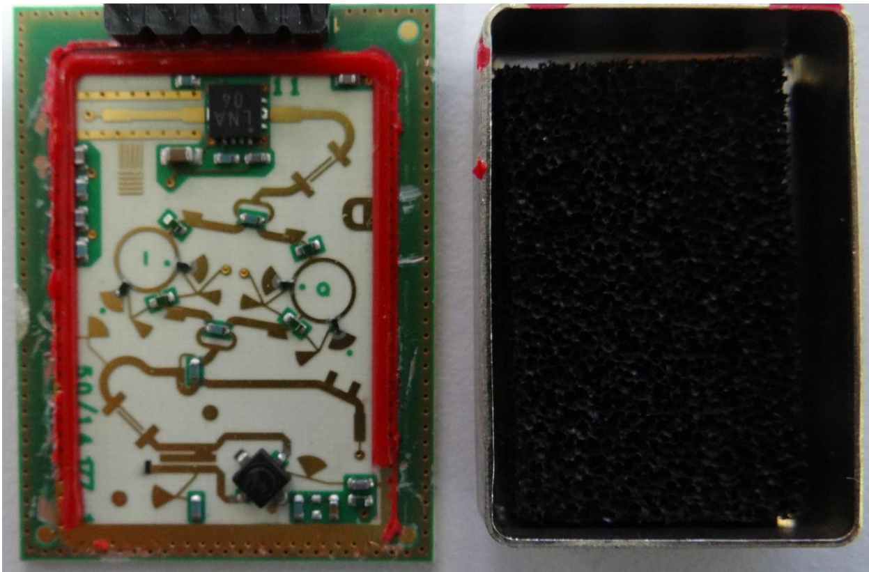
Rear (Screen Can removed)
