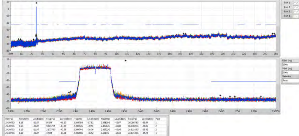
802.11ax HEW20_Nss4,(MCS0)_4TX 2412MHz
