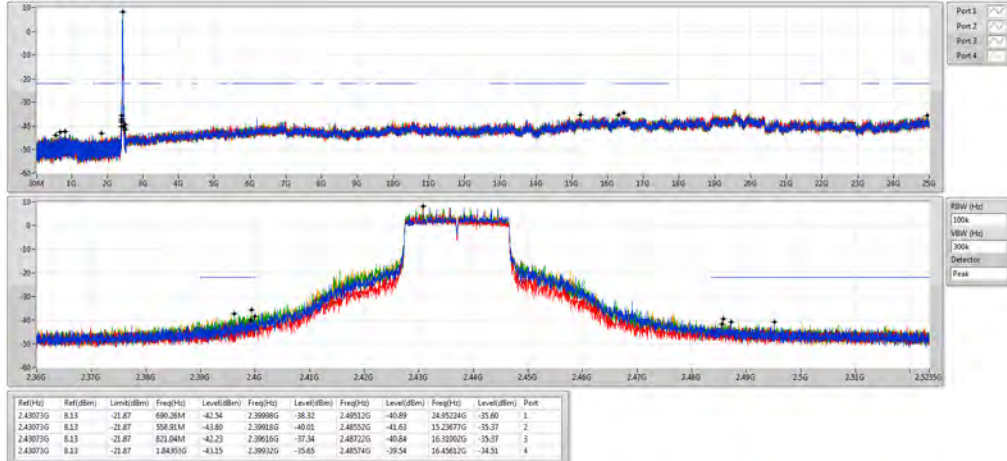
802.11ax HEW20_Nss4,(MCS0)_4TX 2437MHz
