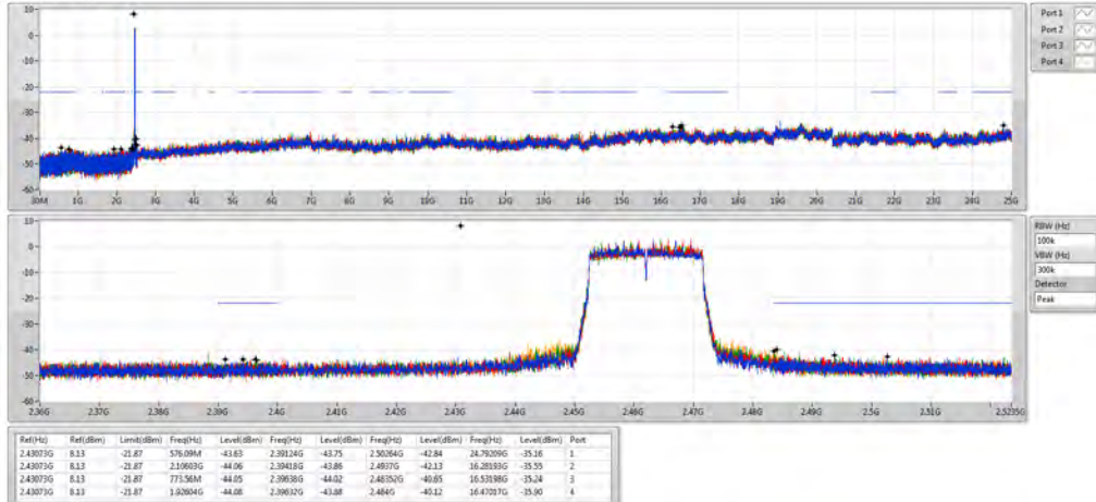
802.11ax HEW20_Nss4,(MCS0)_4TX 2462MHz
