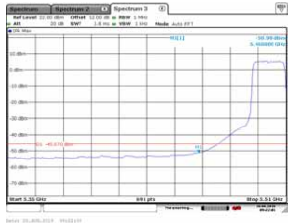
5500MHz with SISO
