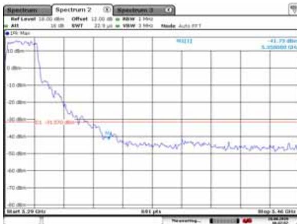
5300MHz with Beamforming
