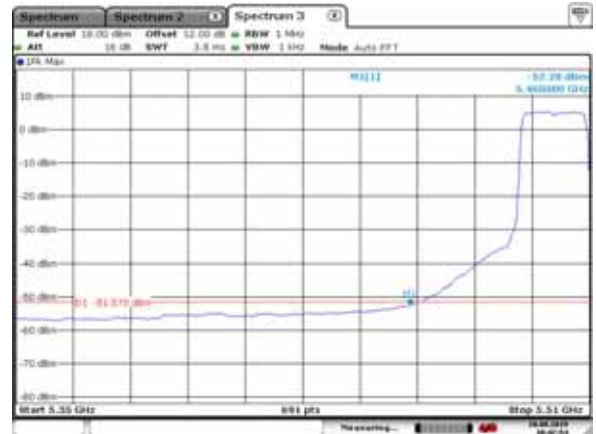
5500MHz with Beamforming
