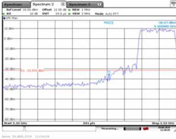
5510MHz with CDD
