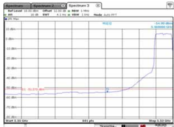
5520MHz with Beamforming
