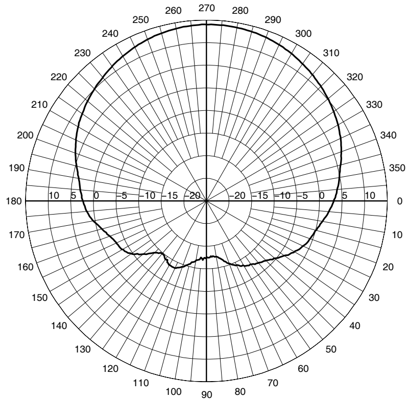
Z2081 Azimuth Cut
