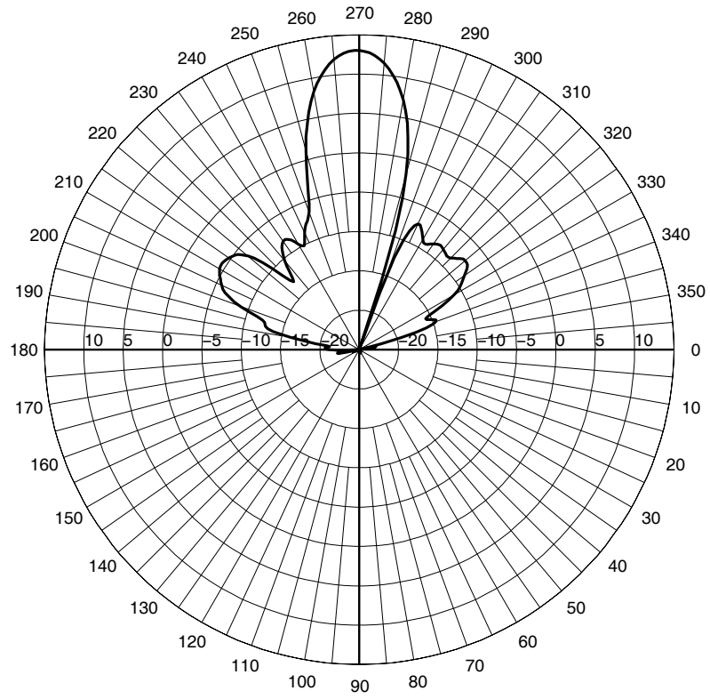
Z2081 Elevation Cut
