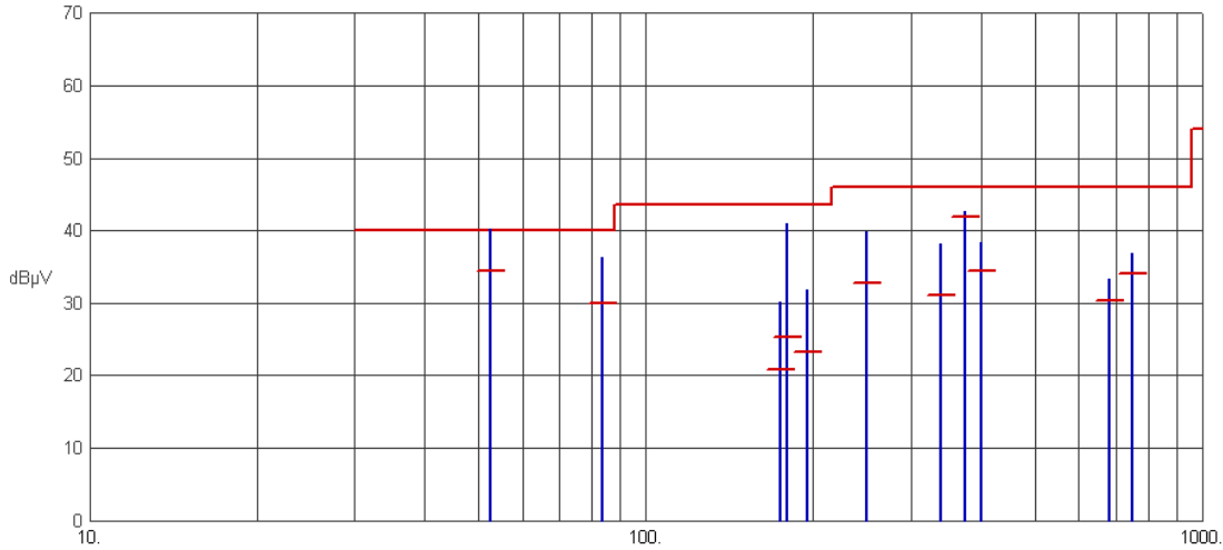
Test No.: 288-12, Radiated Emissions - Horizontal Polarity
