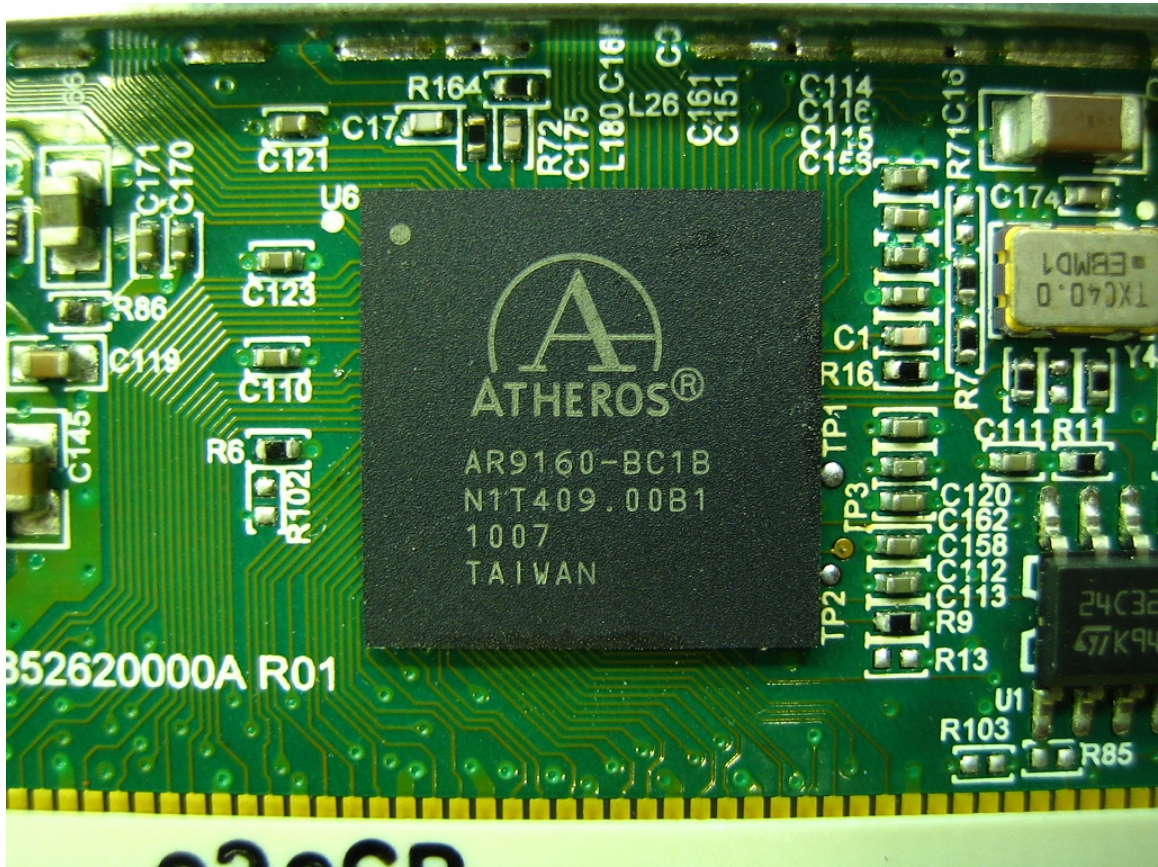
RF Card
