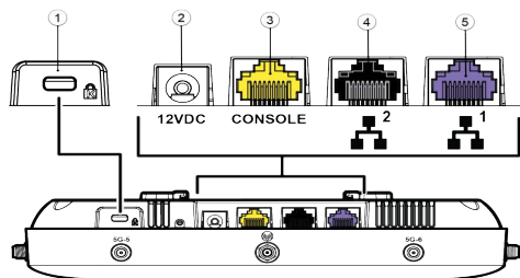
Figure 2 AP510e back ports
