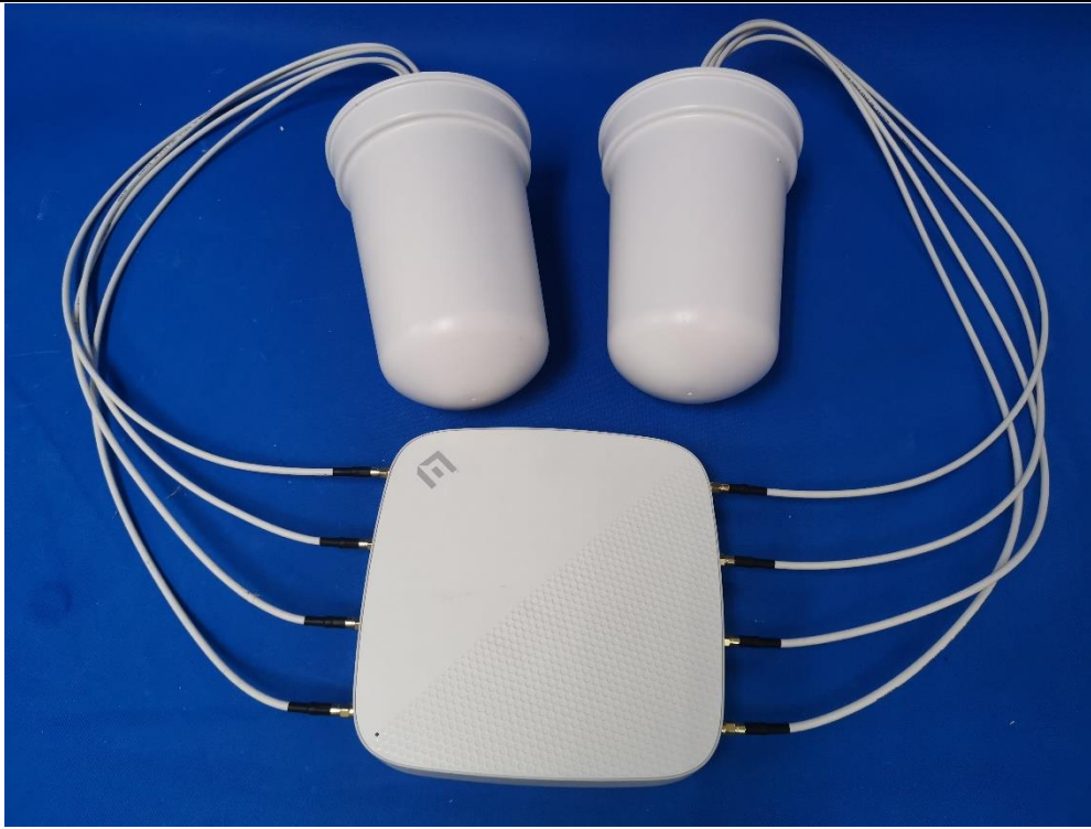
EUT Photo(2) Wireless access point with sector antenna
