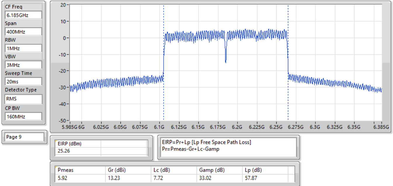
EIRP;Band:6.2G;be160;BWch:160MHz;Nss:1,(M15);Nant:2;Ch:6185MHz;TX
