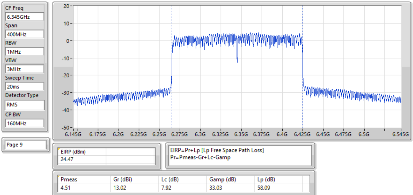
EIRP;Band:6.2G;be160;BWch:160MHz;Nss:1,(M15);Nant:2;Ch:6345MHz;TX
