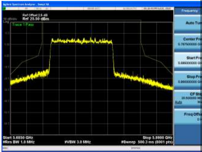
5775MHz with 4*4 Beamforming PK
