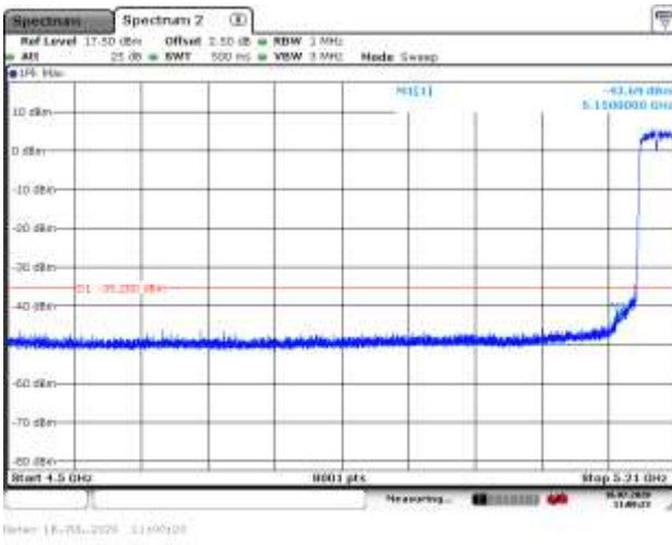
5230MHz with 2*2 Beamforming PK
