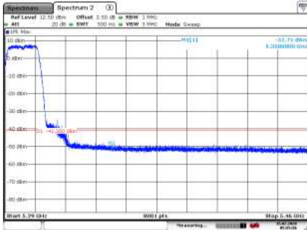
5300MHz with 4*4 Beamforming PK
