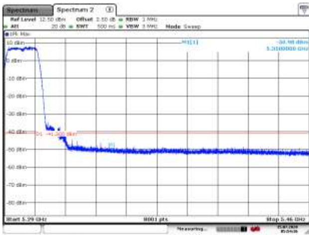
5300MHz with 4*4 CDD PK
