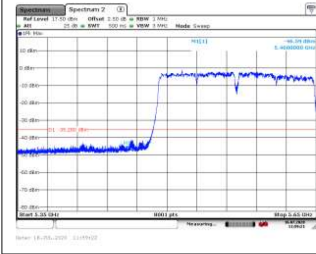
5570MHz with 2*2 Beamforming PK
