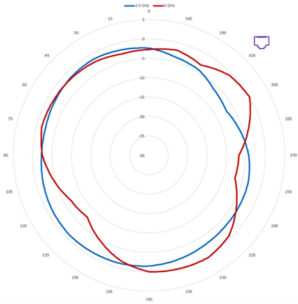
Antenna 3
