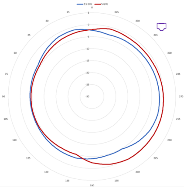
Antenna 4
