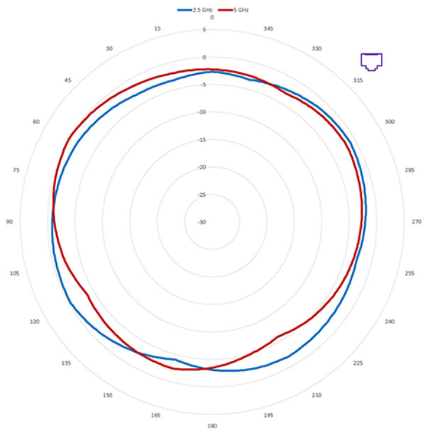
Antenna 2
