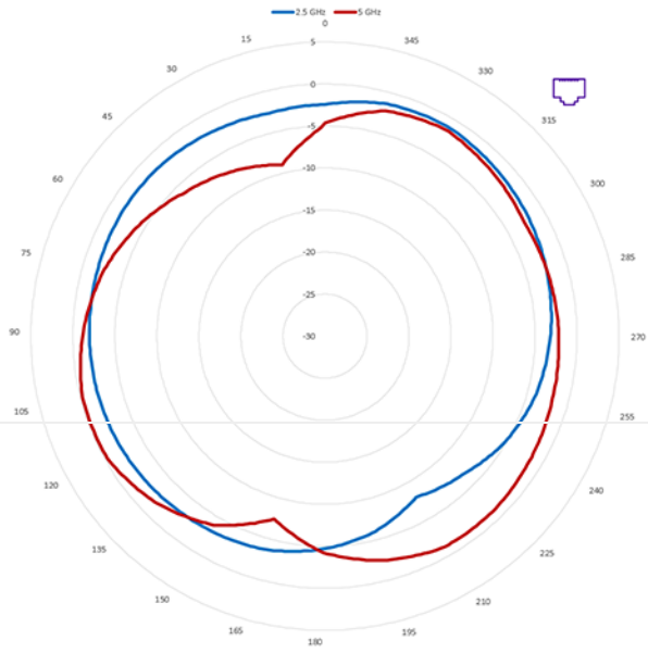
Antenna 1
