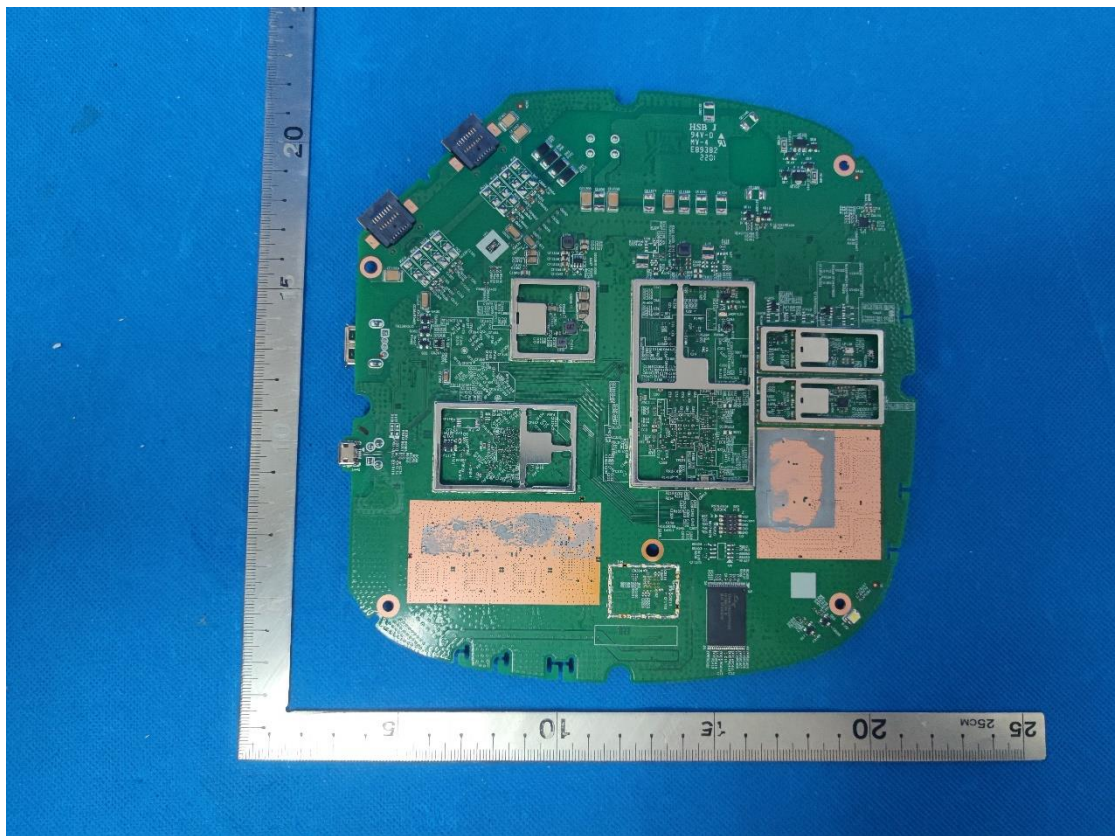
(2) EUT Photo(AP410C)
