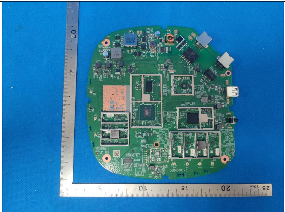
(4) EUT Photo(AP410C)
