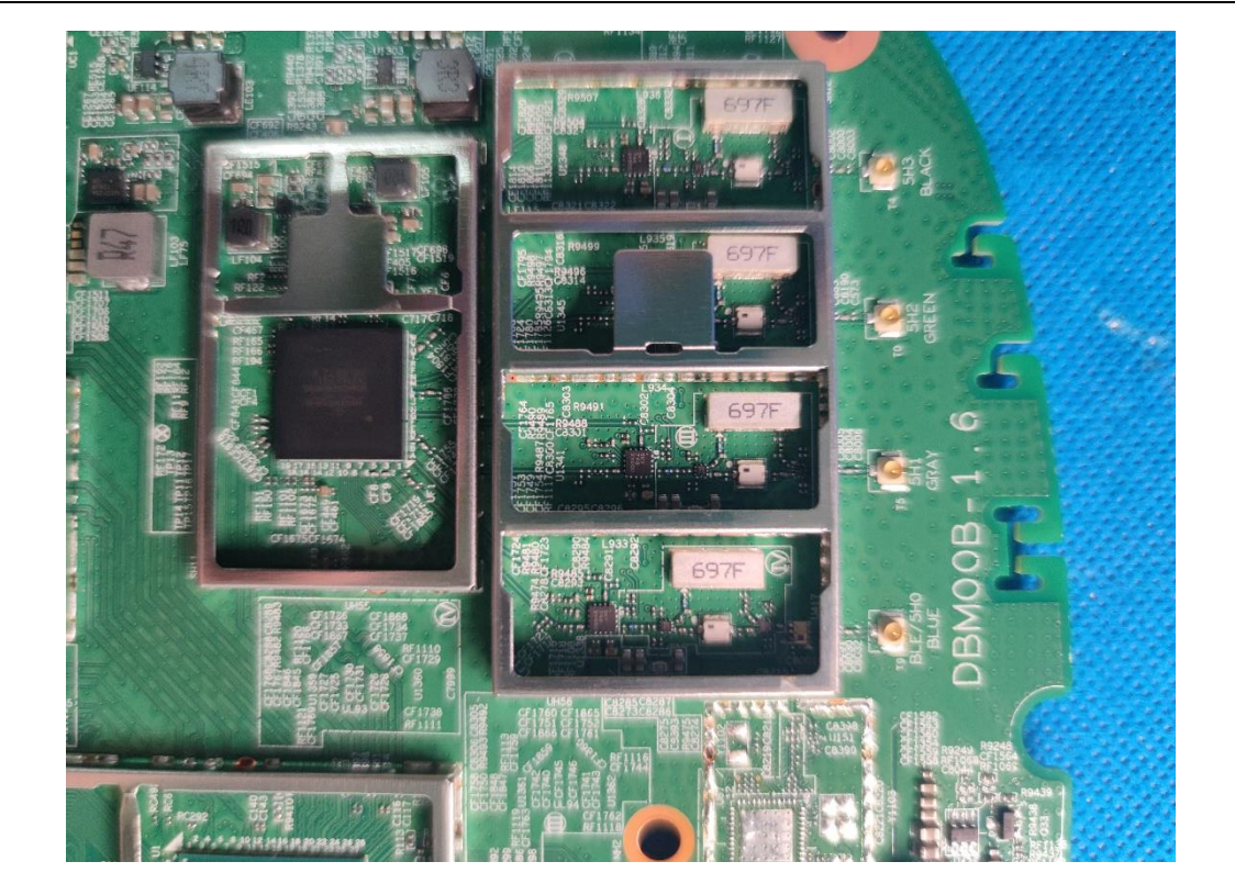
(4) EUT Photo(AP410C)
