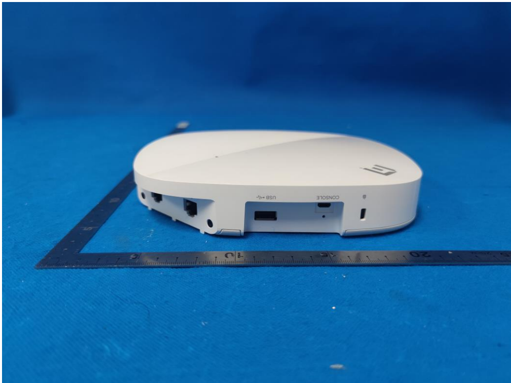
(6) EUT Photo(AP410C)
