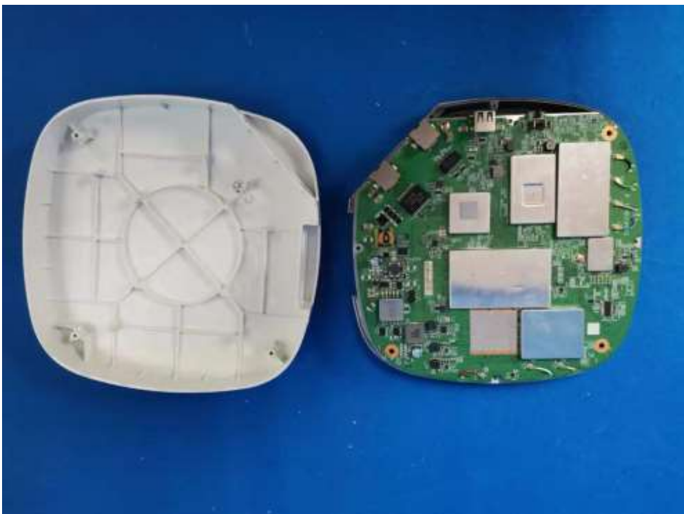
(2) EUT Photo(AP410C)
