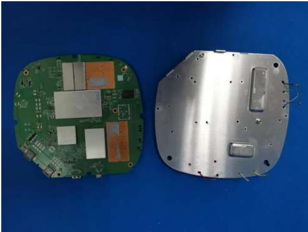
(4) EUT Photo(AP410C)
