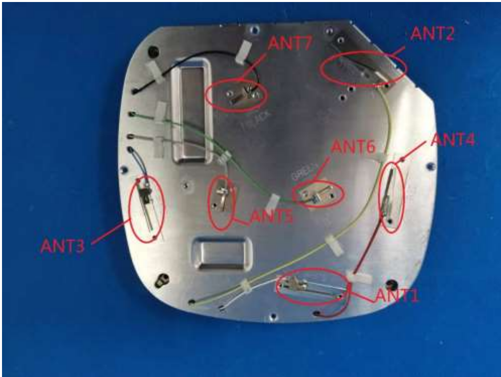
(9) EUT Photo(AP410C)
