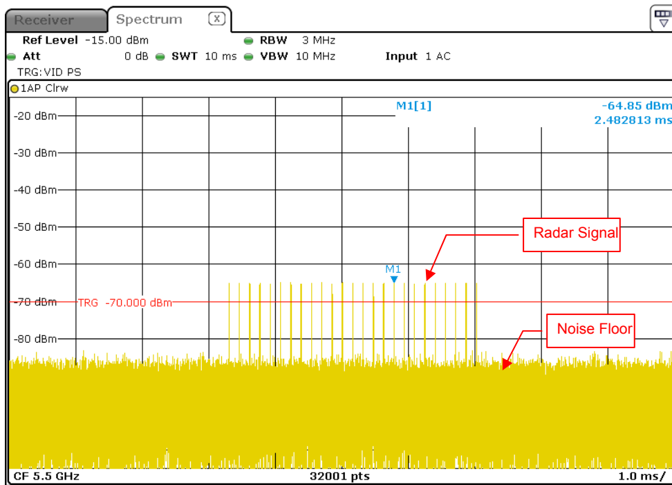
Radar Signal 2
