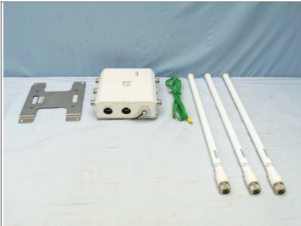
Antenna Part No.: ML-2499-HPA8-01
