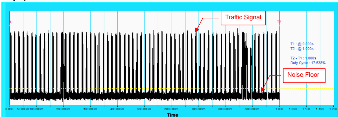
IEEE 802.11ac VHT80 Duty Cycle : 17.538% Duty Cycle
