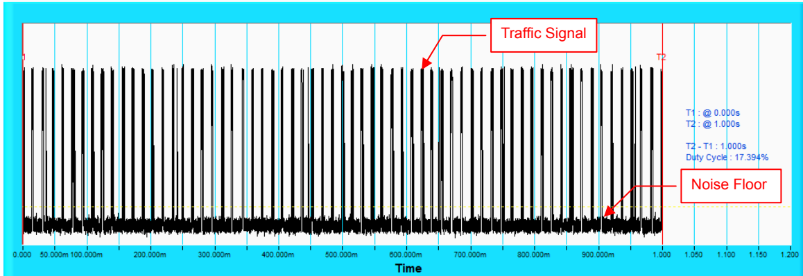
IEEE 802.11n HT20 Duty Cycle : 17.394% Duty Cycle
