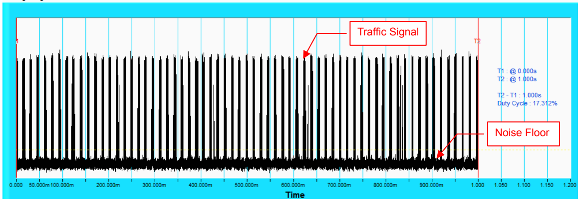
IEEE 802.11n HT40 Duty Cycle : 17.312% Duty Cycle
