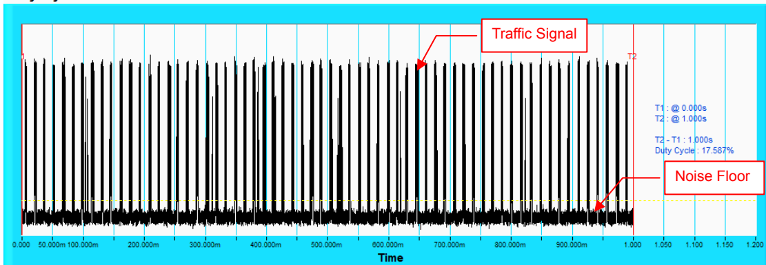
IEEE 802.11n HT40 Duty Cycle : 17.587% Duty Cycle
