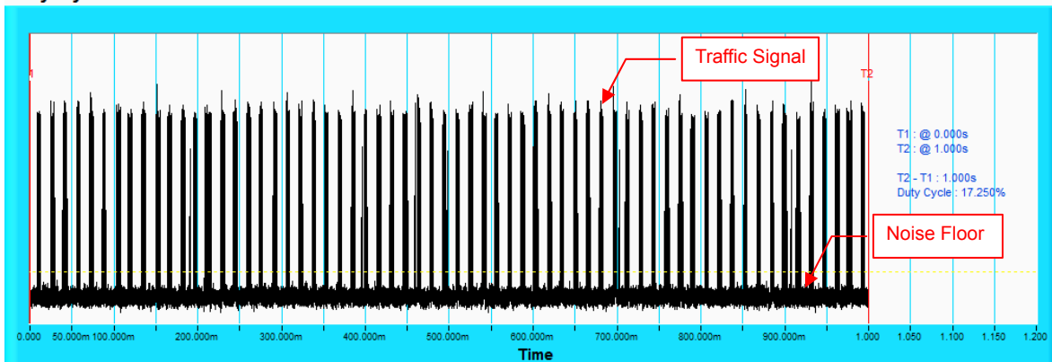
IEEE 802.11ac VHT80 Duty Cycle : 17.250% Duty Cycle
