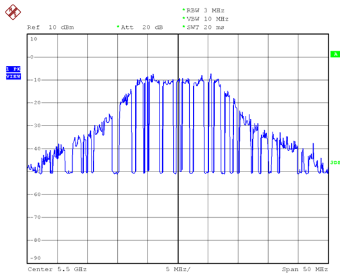
Waveform of EUT links up with Client
