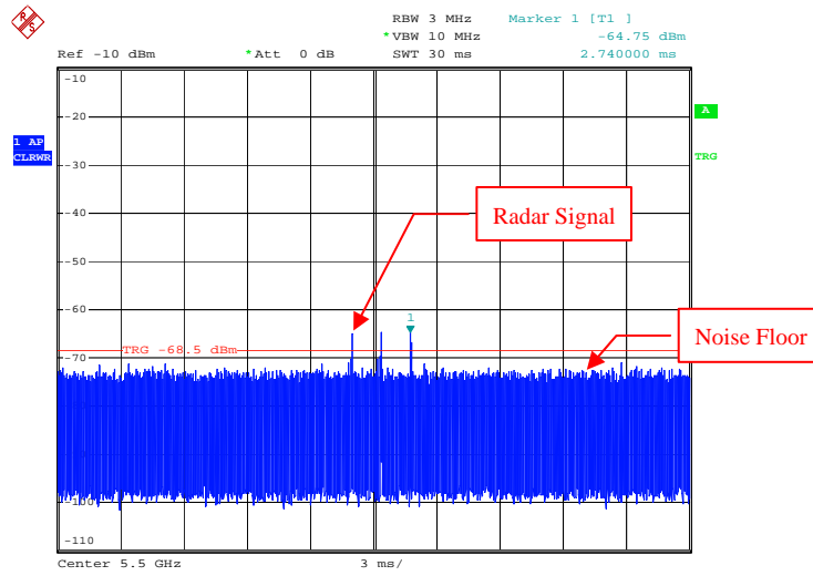
Single Burst of Radar Signal 5
