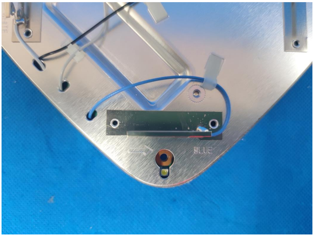
(6) EUT Photo(AP305C)
