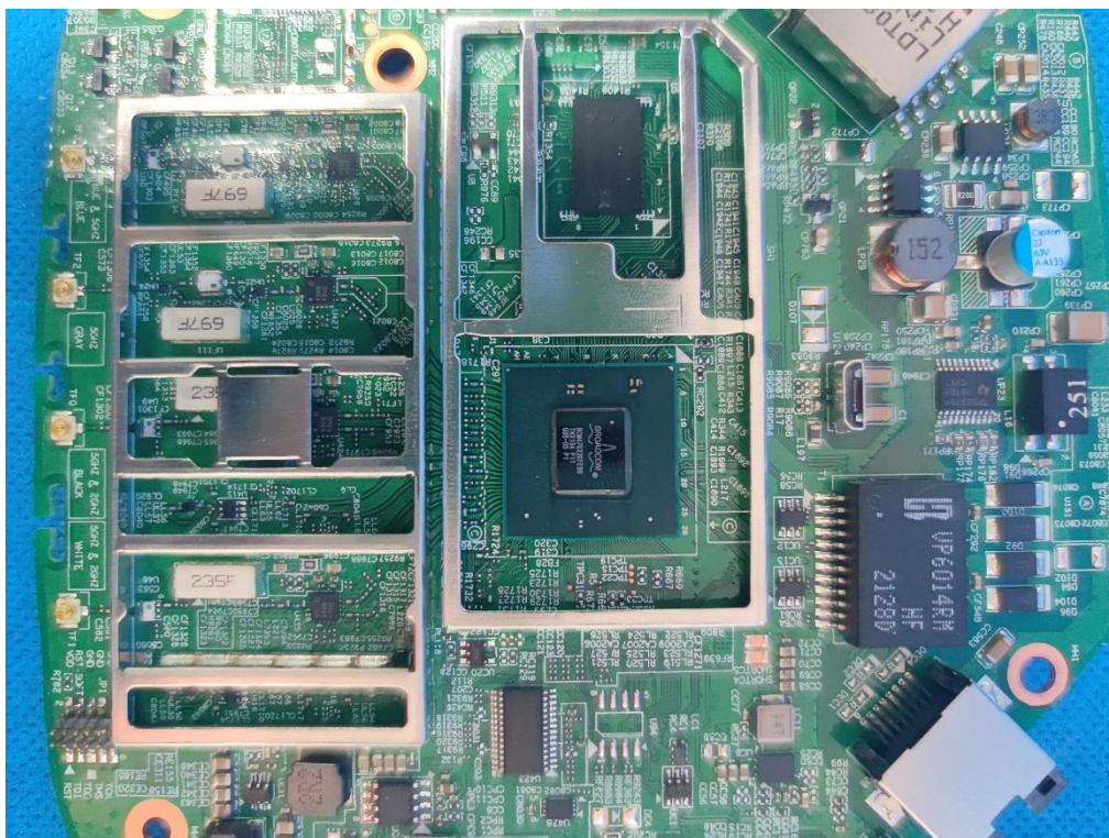
(4) EUT Photo(AP305C)
