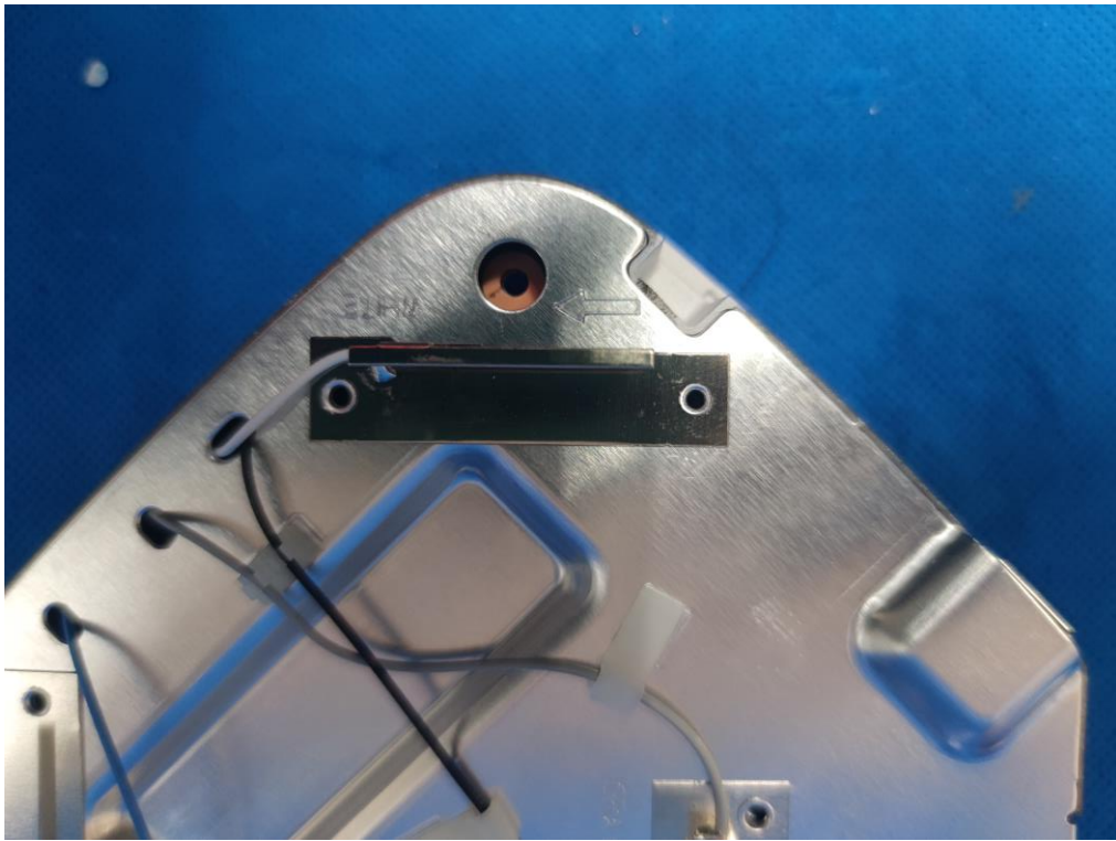
(9) EUT Photo(AP305C)
