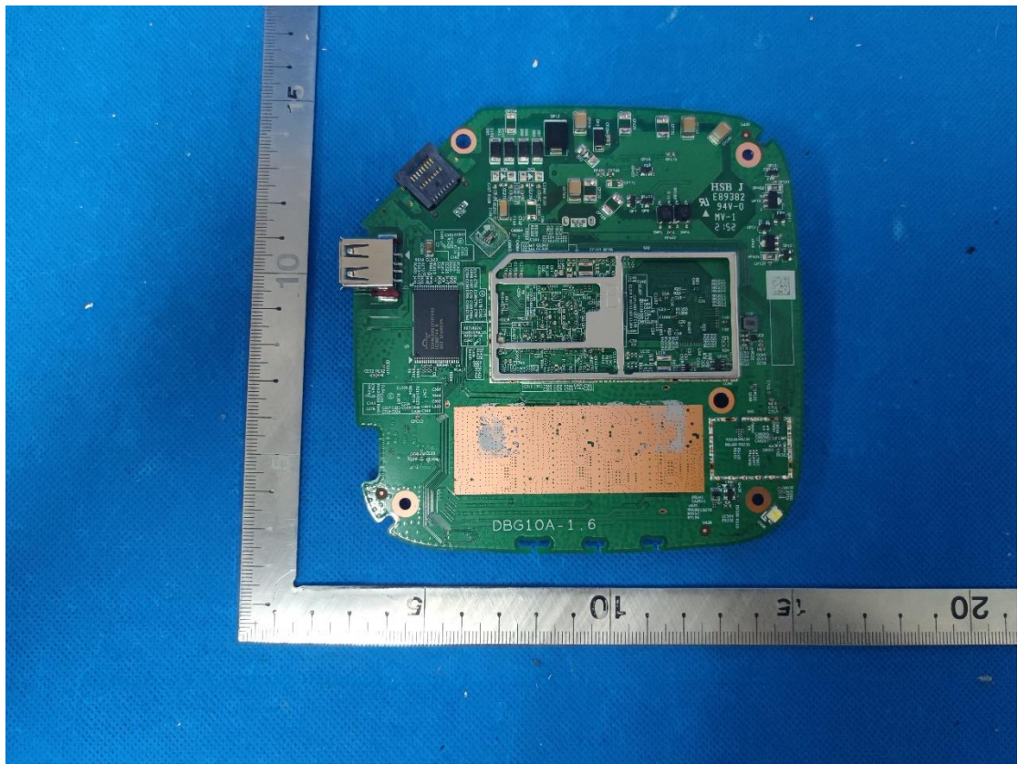
(2) EUT Photo(AP305C)
