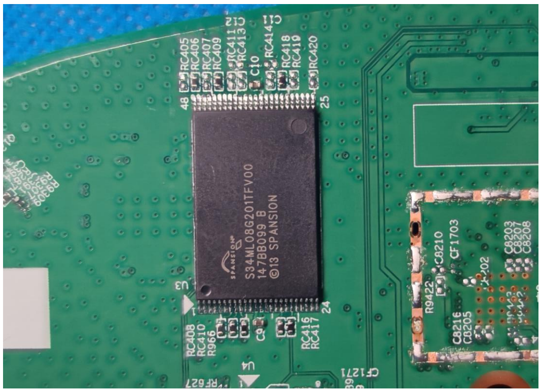
(6) EUT Photo(AP305C)
