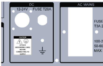
Figure 2: Location earthing label on R60 VDES Base Station
