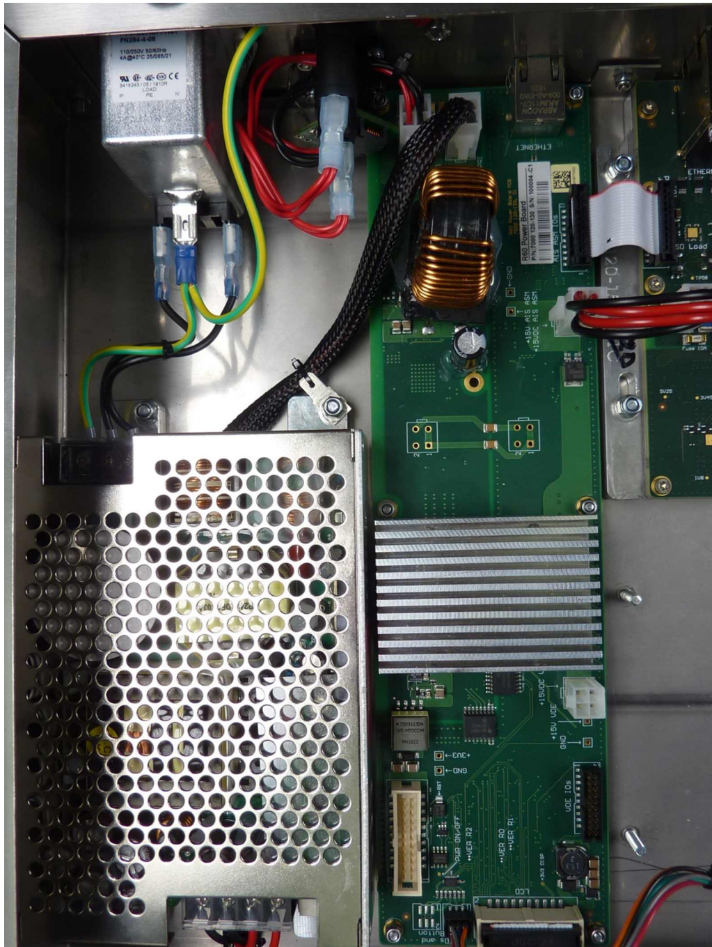
R60 VDES Base station, power supply, power board, power filter
