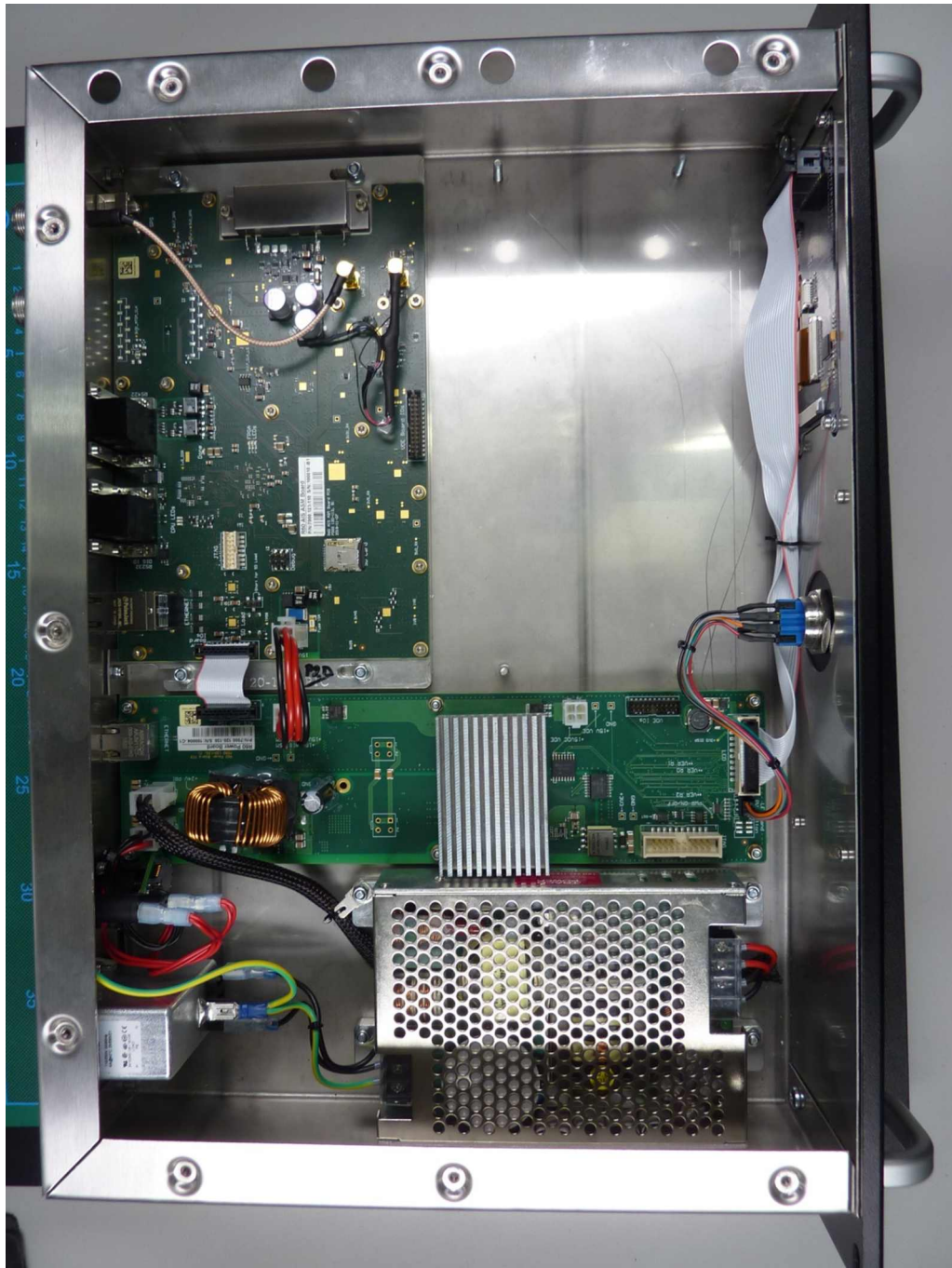
VDES Base station, internal view, cover removed
