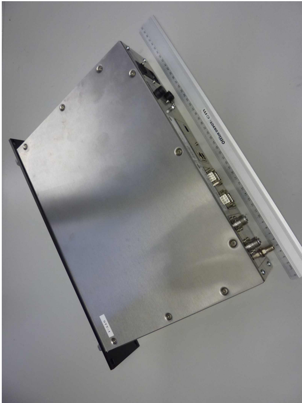
R60 VDES Base station, 3-D-view 2
