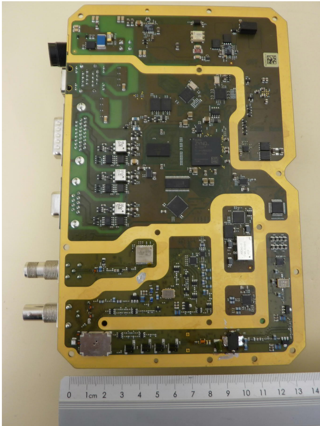
PCB test sample 1, bottom view
