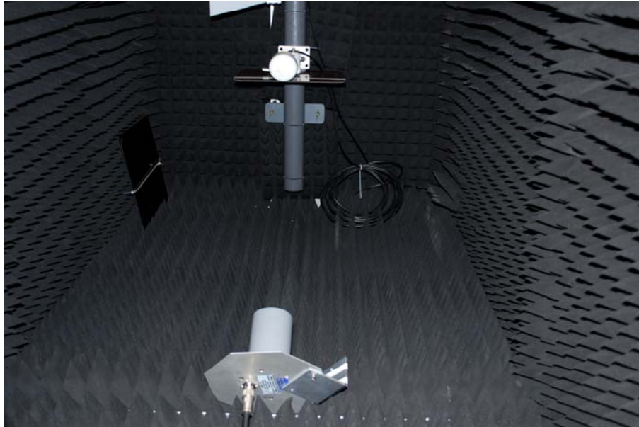
L-Band interference test – GPS Antenna Unit 2
