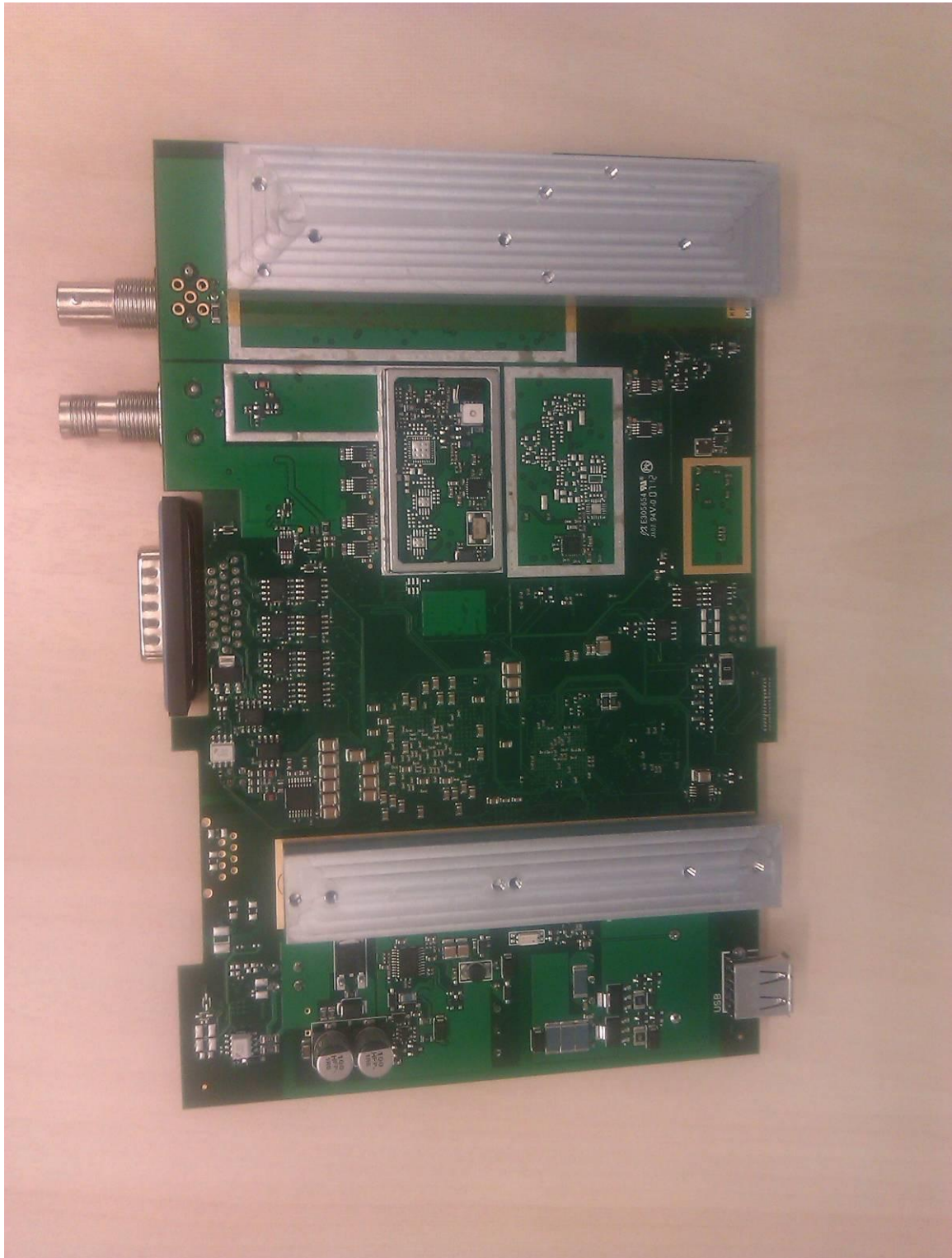
Photograph 5: - PCB bottom view (shielding removed)
