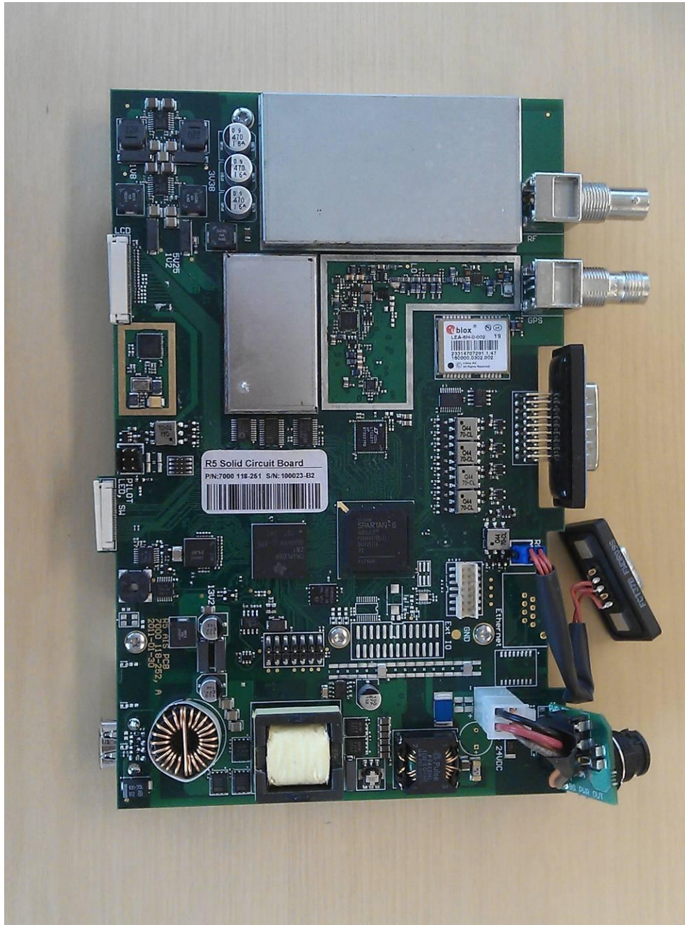
Photograph 1: - PCB top view
