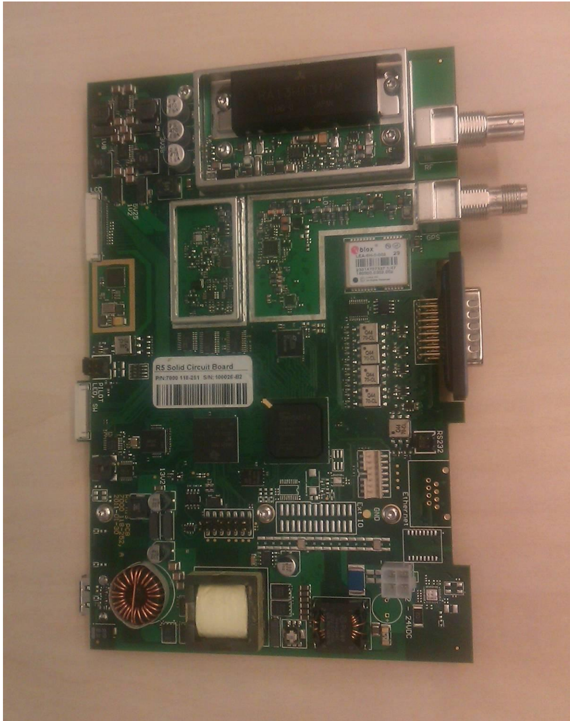
Photograph 2: - PCB top view (shielding removed)
