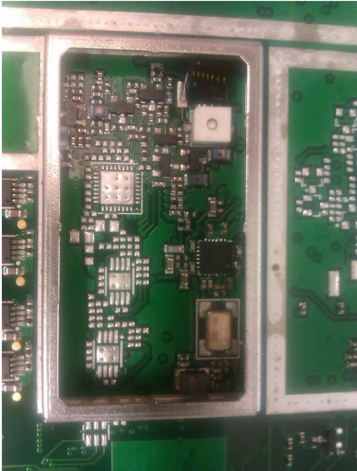
Photograph 6: - Detail of bottom view (shielding removed)
