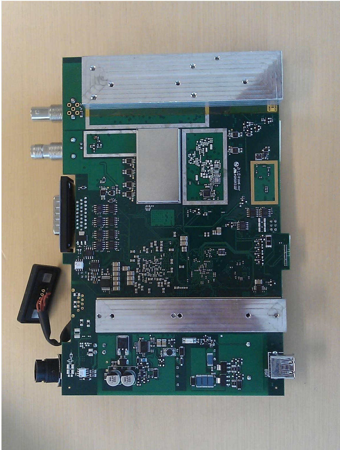
Photograph 4: - PCB bottom view
