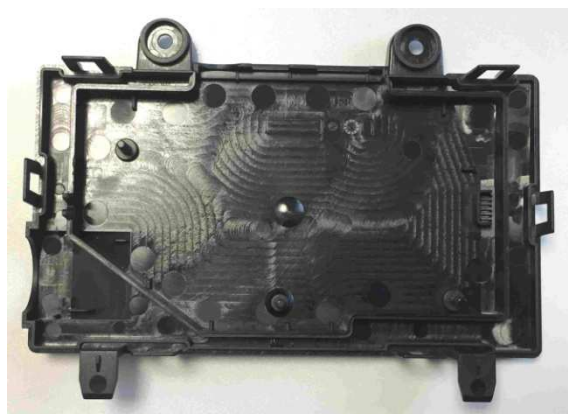
Bottom Housing, view inside the Part.
