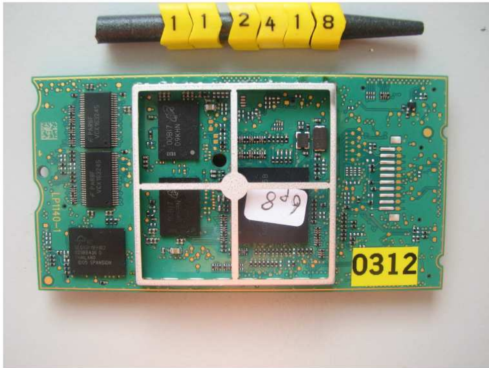
Core PCB top view (metal shield removed)
