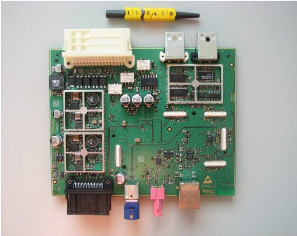
Main PCB top view (metal shields removed)
