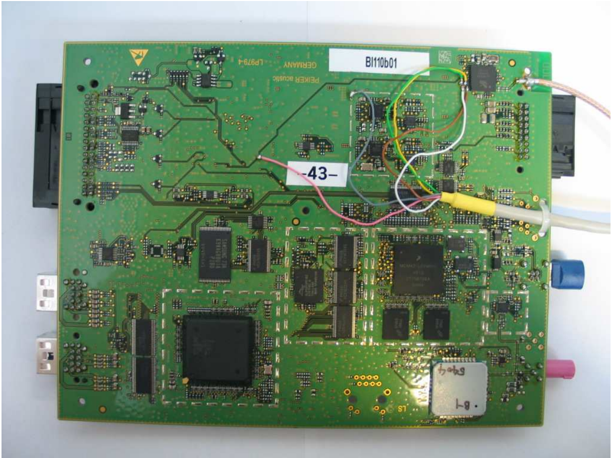
Photo 9: EUT (internal, rear side)
