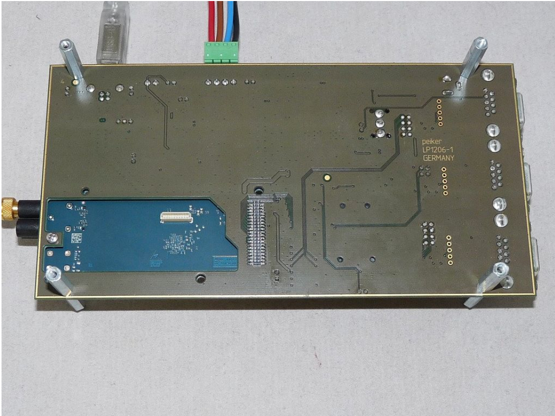
Photo 5: OUT setup (OUT and auxiliary equipment, rear side)
