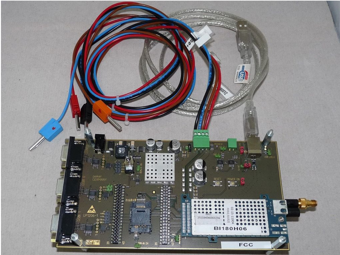
Photo 4: OUT setup (OUT and auxiliary equipment, front site)
