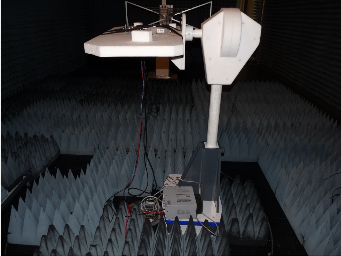
Photo 2: Test setup for radiated tests, spurious emissions acc. to FCC Part 22, 24 and IC RSS-Gen (above 1 GHz)
