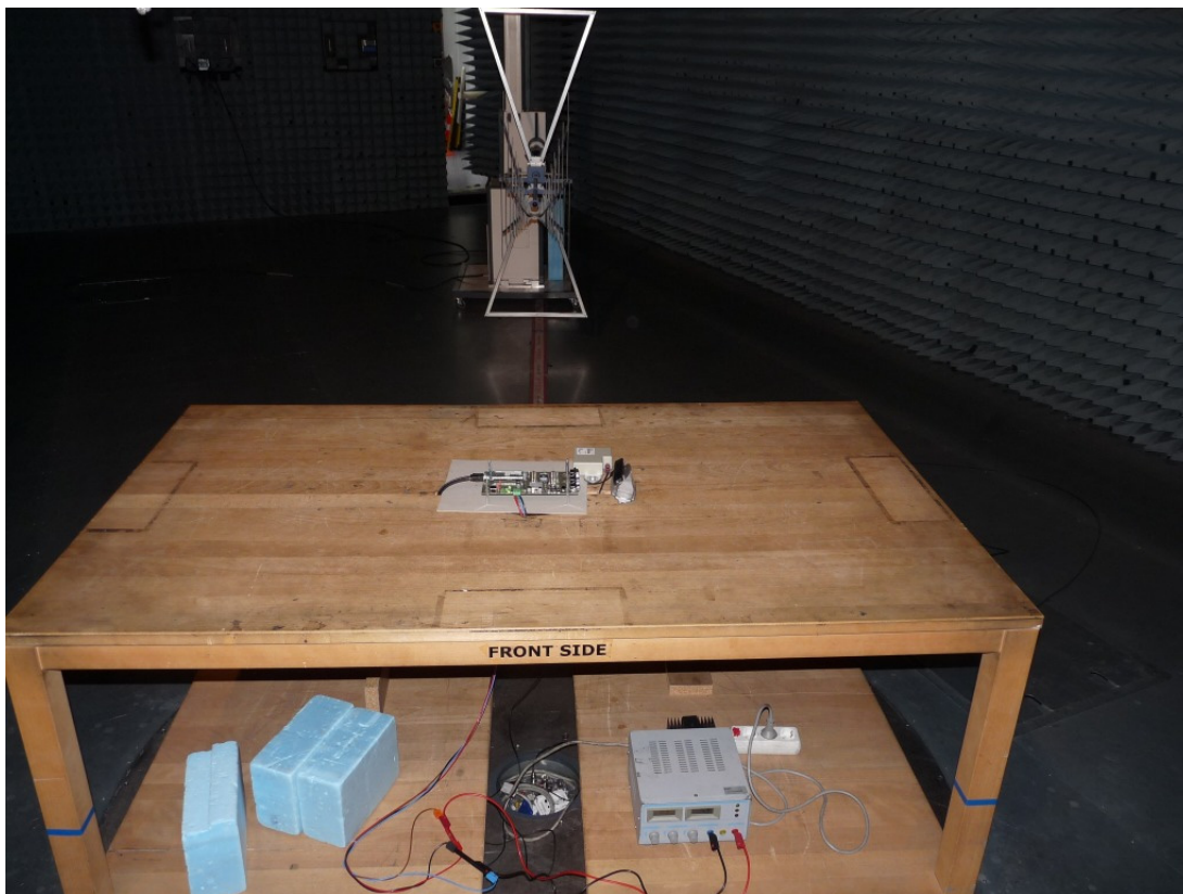
Photo 3: Test setup for measurements up to 1 GHz acc. to IC RSS-Gen
