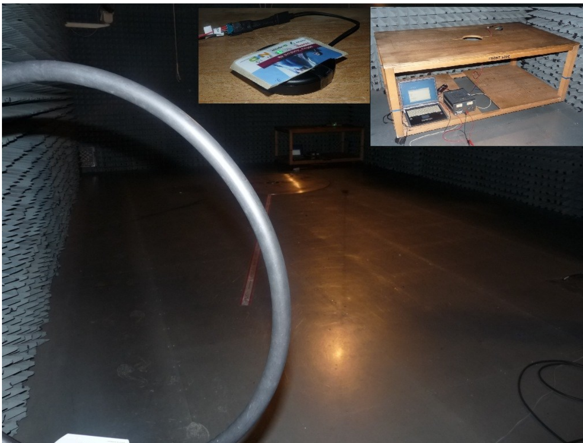
Photo 1: Test setup for spurious radiated emissions measurements (Enclosure, semi-anechoic chamber, 9 kHz to 30 MHz, unintentional radiator §15)
