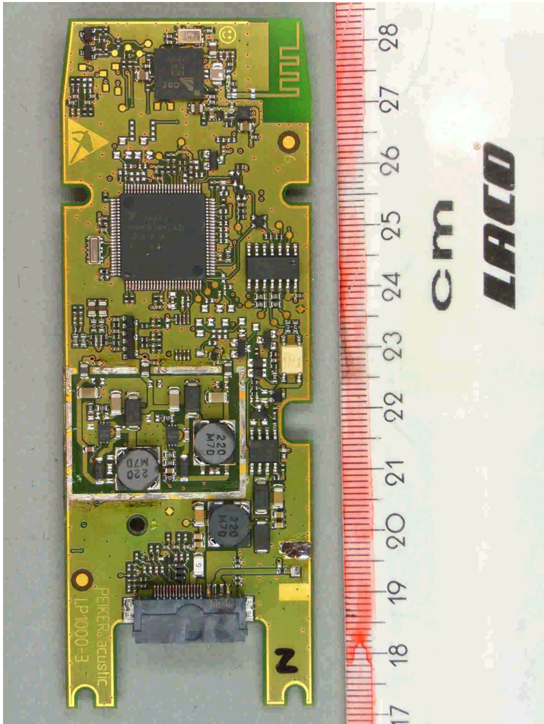
81099_12.jpg CKIV, PCB, top view, cover removed
