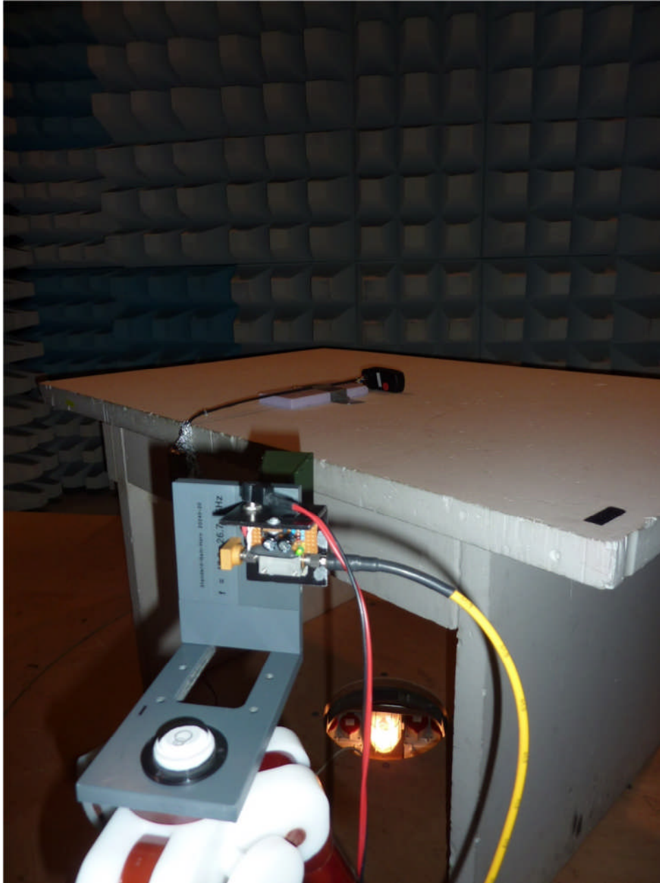
113907_18 Test setup fully anechoic chamber
