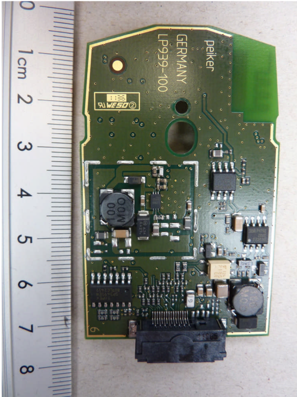
113907_06: CKIII-HFP4, internal view 1
