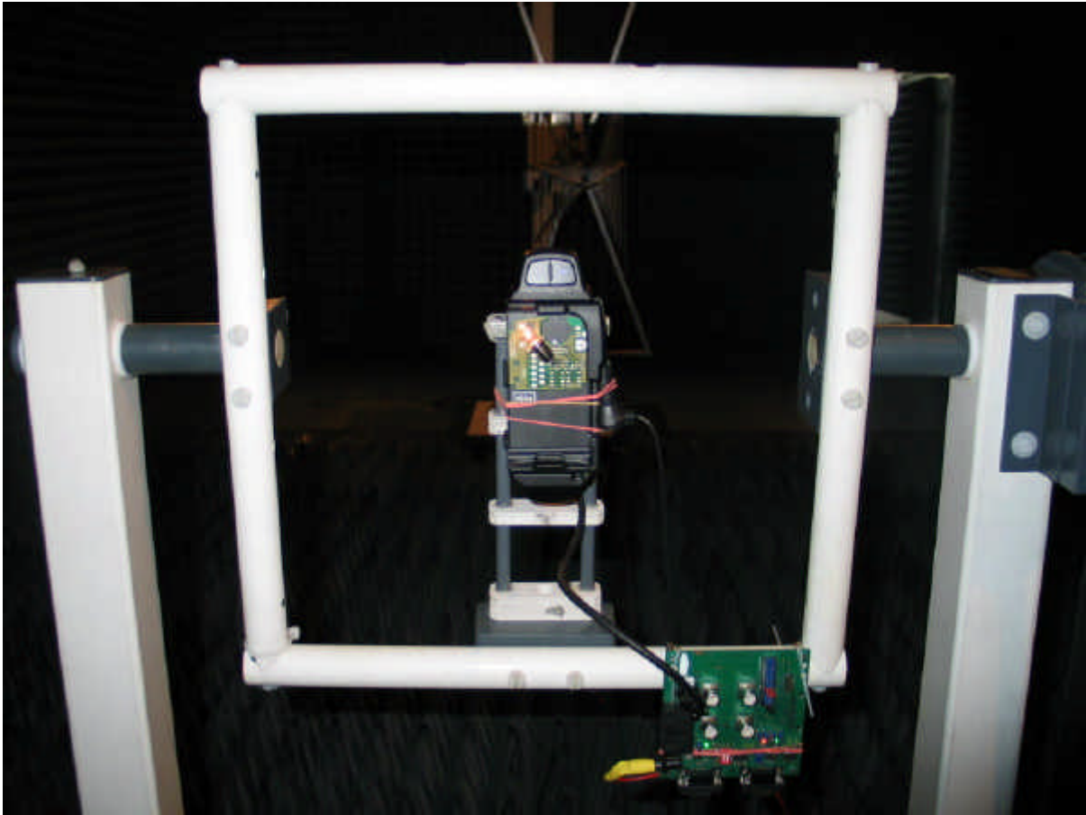
PHOTO No. 3: EUT and COM port adaptor, setup used for radiated measurements
