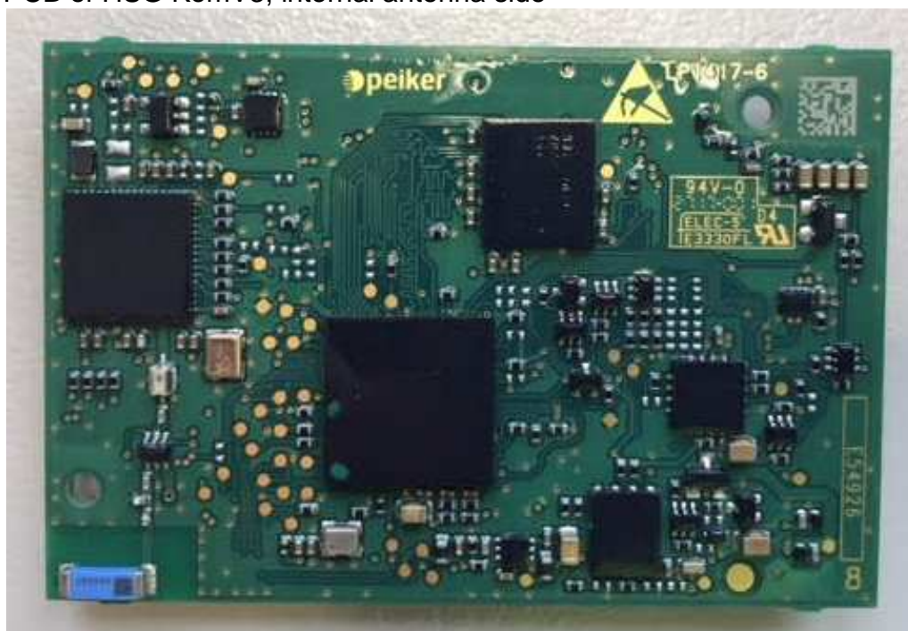
PCB of HSG KomV3, internal antenna side
