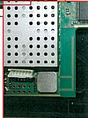
picture2: Print-F Antenna
