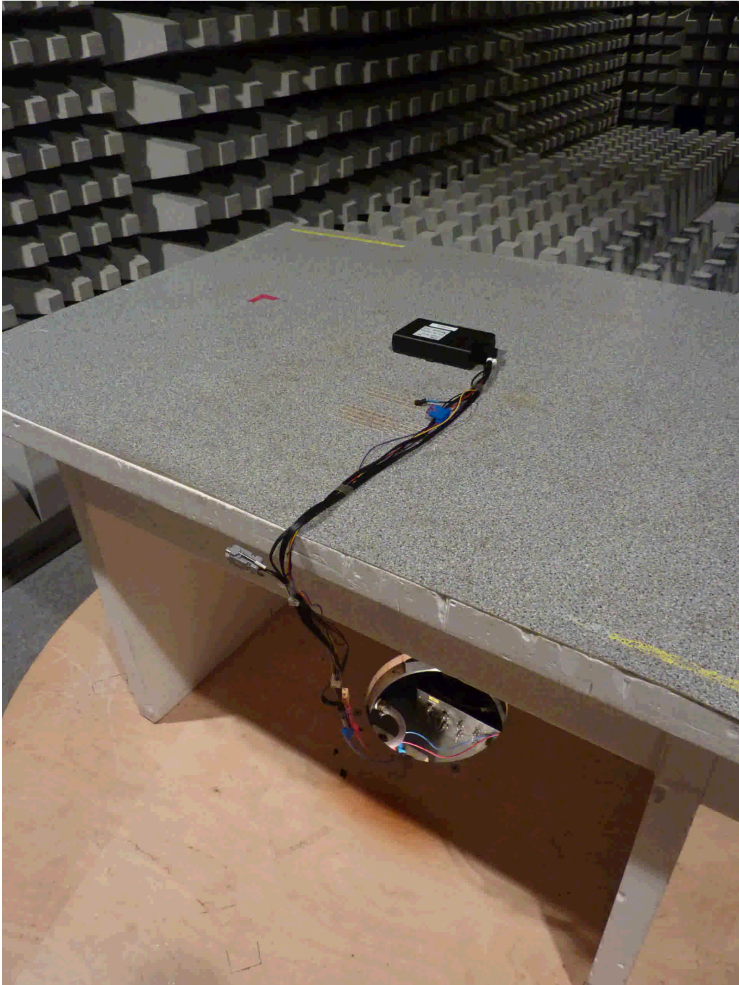
100798_11.jpg CIB FSE iPhone, test set-up fully anechoic chamber
