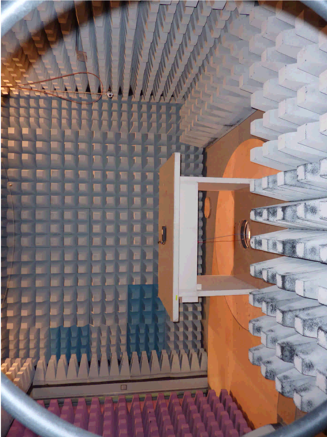
100798_13.jpg CIB FSE iPhone, test set-up fully anechoic chamber
