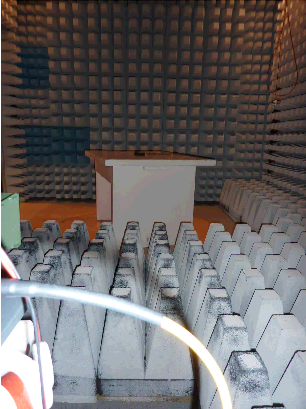
100798_12.jpg CIB FSE iPhone, test set-up fully anechoic chamber
