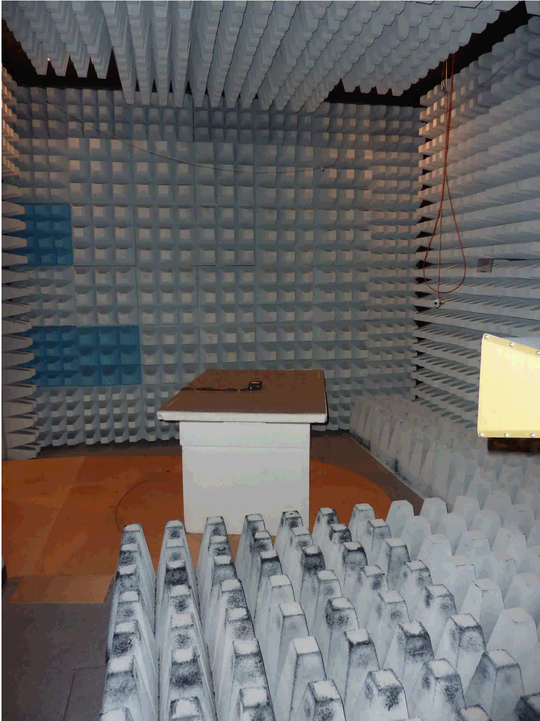
100798_10.jpg CIB FSE iPhone, test set-up fully anechoic chamber
