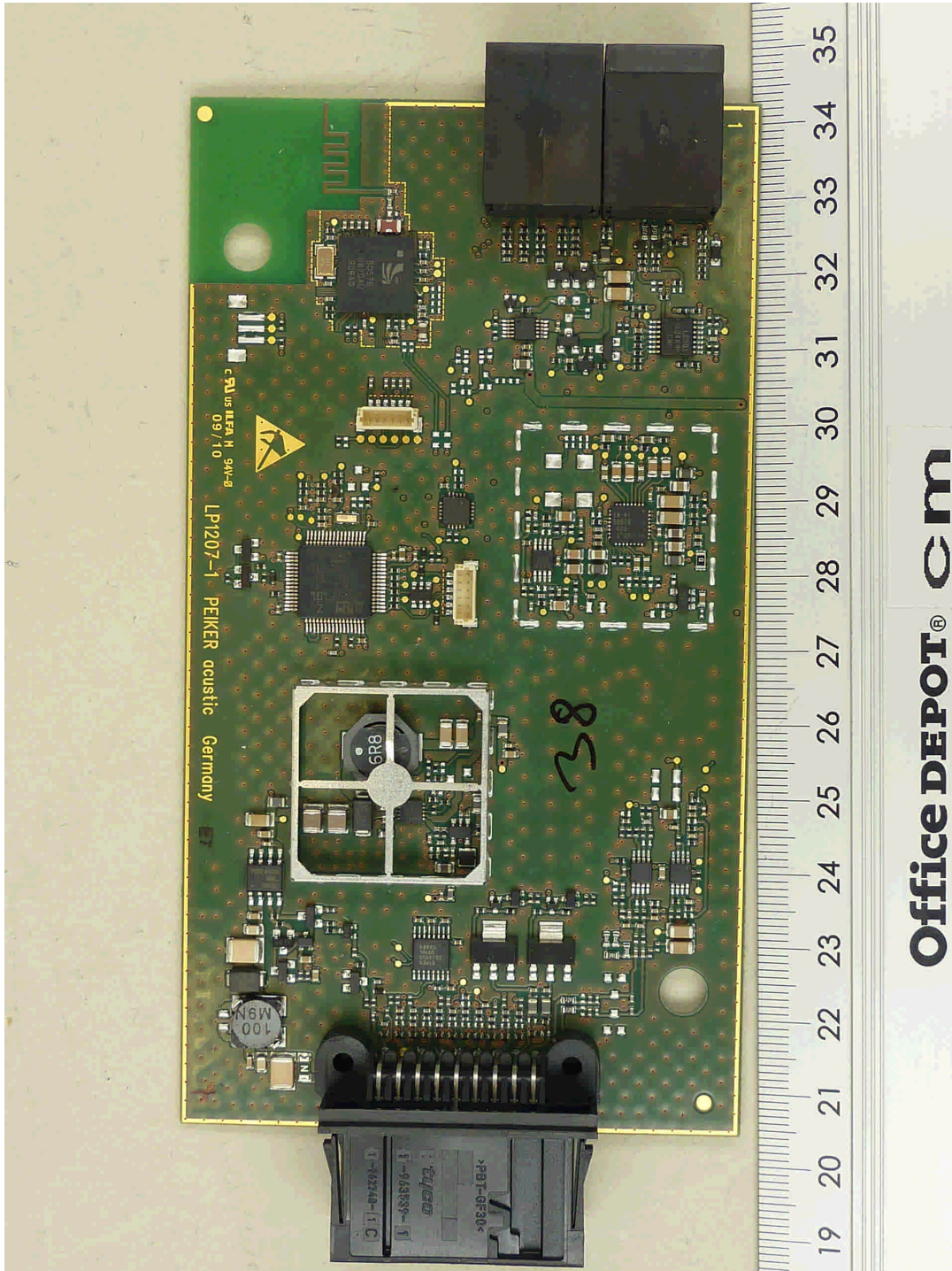
100798_g.jpg CIB FSE iPhone, PCB, top view, shielding removed
