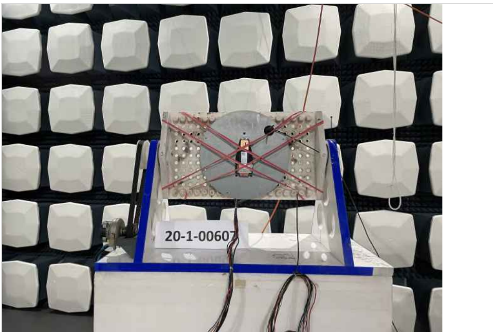
Photograph 2: EUT Test Setup in the anechoic chamber, Radiated emissions
