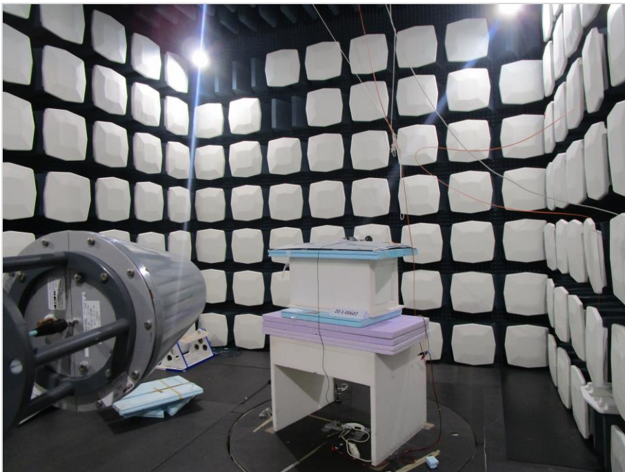
Photograph 4: EUT Test Setup 2 in the fully anechoic chamber, overview
