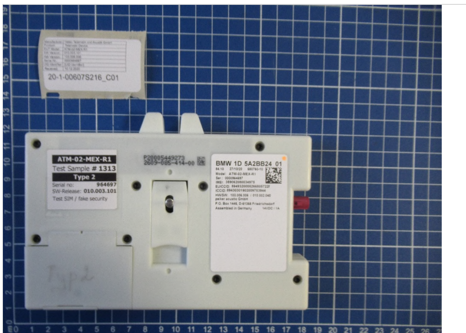
Photograph 2: EUT Top view
