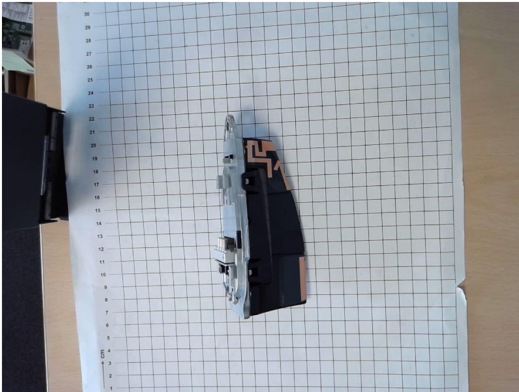
Photograph 5: Roof Antenna
